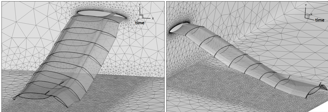
Figure 14. Spacetime mesh for landing case, i.e. aerfoil with a slat and flap deployment followed by an increase of its angle of incidence and a spoiler deployment which, in turn, decreases the incidence, all of which happens while approaching to the ground.
