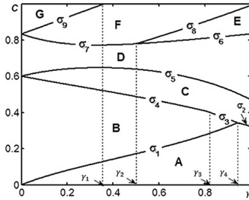
Fig. 4. Strategy choices in Model D.
