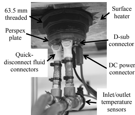
Fig. 7. External view of bulkhead connector (fluid, power).
