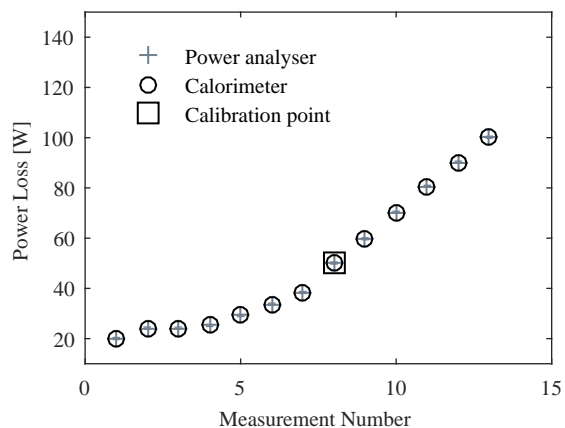
Fig. 13. Absolute power measurements including one calibration point.
