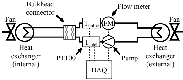
Fig. 9. Schematic of the calorimeter fluid cooling system.
