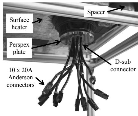
Fig. 8. External view (DUT connections).
