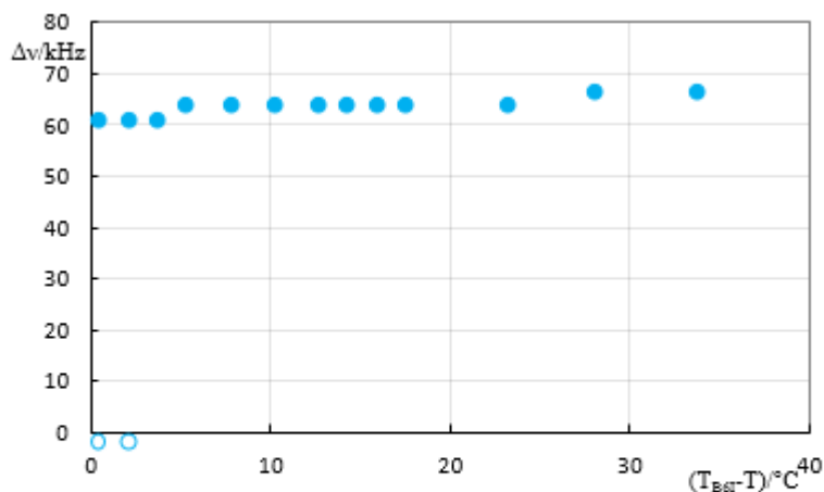
Figure 18. (colour online) The dependence of the quadrupolar splitting, \Delta\nu_{CD} , on the shifted temperature (T_{B_{6I}} - T) for 6O.7.O6 doped with 2.7wt % CB7CB-d 4 . Here \circ indicates the isotropic peak in the biphasic region and \bullet denotes the quadrupolar splitting in the biphasic region and across the B 6 phase.
