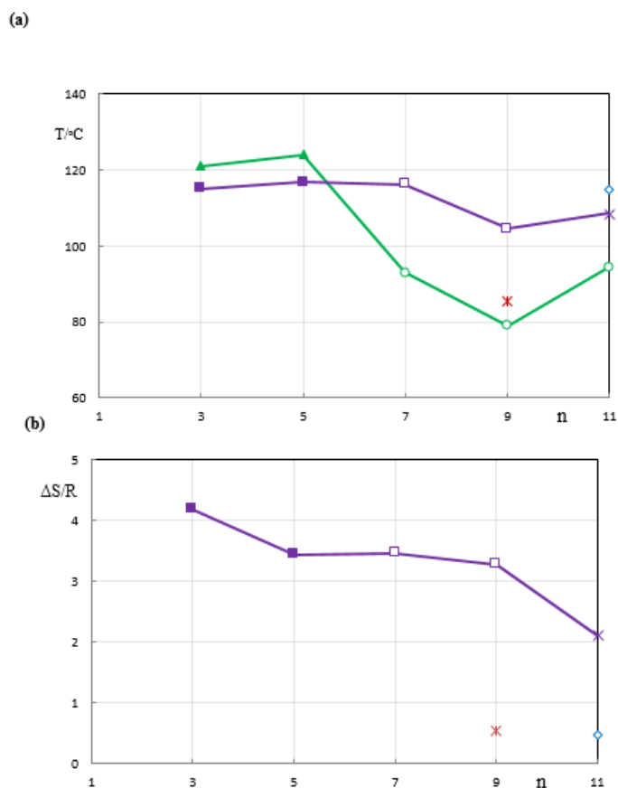
Figure 7 (colour online) Dimers 6O.n.O6 (a) The dependence of the transition temperatures, T_i , on the length of the alkane spacer, n and (b) the dependence of the scaled transitional entropies, \Delta S/R , also on n . The symbols used to denote the temperatures and transitional entropies are \blacktriangle for Cr - I; \circ for Cr - B_6 or, for n=9 , B_6 - Cr; \blacksquare for ( B_6 - I); \square for B_6 - I; \times for ( B_6 - B_6 ); \times for B_6 - N; \diamond for N - I. Here (\ ) denotes a monotropic transition.
