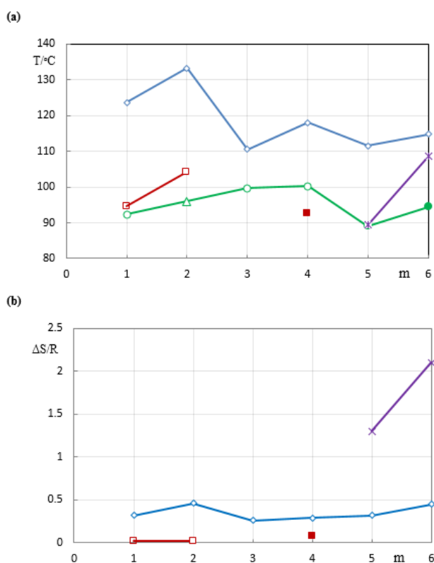
Figure 12. (colour online) The dependence of (a) the transition temperatures, T_i and (b) the scaled transitional entropies, \Delta S/R , on the number of carbon atoms, m , in the terminal alkyloxy chains for the dimers mO.11.Om . The symbols used to denote the transition temperatures and transitional entropies are \bullet for Cr- B_6 ; \Delta for Cr- N_{TB} ; \circ for Cr-N; \times for B_6 -N; \square for N_{TB} -N; \blacksquare for (N_{TB} -N); \diamond for N-I.
