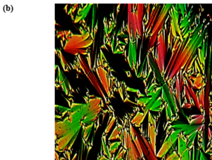
Figure 6. (colour online) The optical textures for the dimer 4O.3.O4 for (a) the jagged bâtonnet in the biphasic region at 105°C prior to the B 6 phase and (b) the fan-like texture at 102°C.
