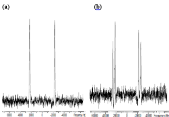
Figure 15. The ^2\text{H} NMR spectra of 2O.7.O2 doped with 3wt % CB7CB- d_4 (a) in the N phase at 102 °C and (b) in the N_{\text{TB}} phase at 86.5 °C.
