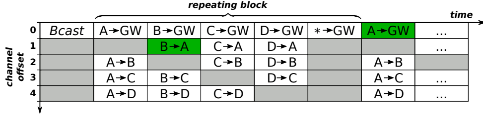
Figure 4: A fragment of the slotframe for networks with 4 forwarding nodes , such as in Fig. 1 and Fig. 5. GW denotes the gateway node, A , B , C , D denote forwarding nodes. Bcast marks a timeslot reserved for broadcast. * → GW denotes a shared slot, in which all nodes directly connected to the gateway are allowed to transmit. The two green cells in the schedule mark one way how to forward a packet from B to the gateway ( GW ), assuming network as in Fig. 5a.
