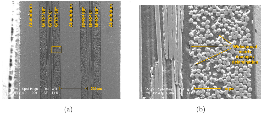
Figure 10: SEM of splice specimens along section 1 (side of specimen), with magnifications of (a) 100× and (b) 1000×.
