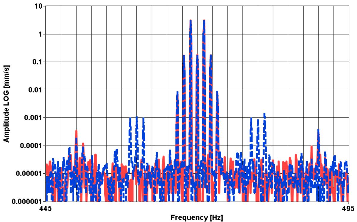
Figure 5: Appearance of additional sidebands as a consequence of damage. Blue dashed line is the damaged case and the undamaged case is the solid red line
