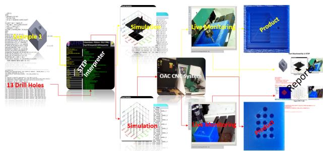
Fig. 7 Experimental setup
