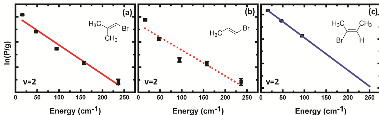
Fig. 7 Boltzmann plots of the rotational population of HBr ( v=2 ) from the photodissociation of (a) BMP-3, (b) EBP-34, and (c) EBB-44 against energy of the HBr( v=2 ) rotational level probed. The population intensities ( P ) are the integrated areas of individual peaks in the REMPI spectrum without any correction for the REMPI line strengths. The degeneracies of the rotational levels are denoted by g . The straight lines (solid, red), (dotted, red) and (solid, blue) are linear fits.
