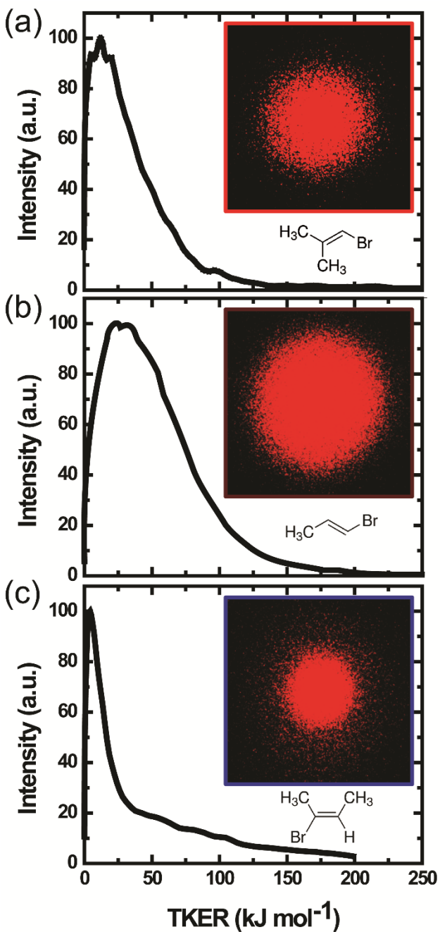
Fig. 3 Velocity map images of HBr ( v=2, J=1 ) fragments from 193-nm photolysis of three methyl-substituted vinyl bromides: (a) BMP-3, (b) EBP-34 and (c) EBB-44) and the derived TKER distributions, averaged over all recoil angles.
