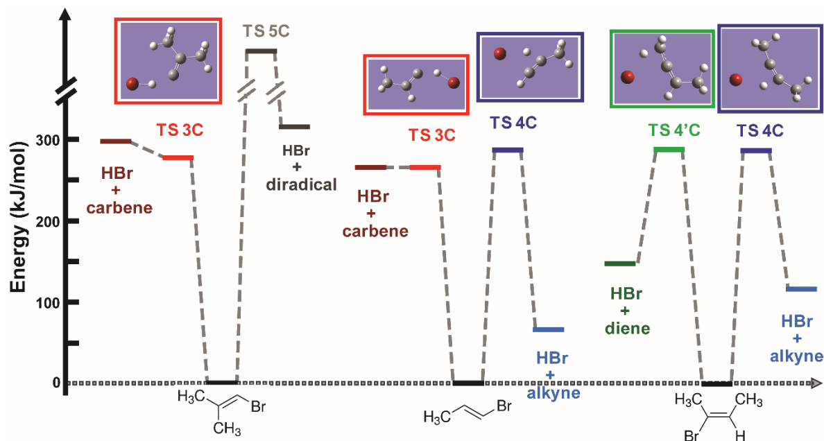
Fig. 2 Zero-point-energy corrected CCSD(T)/aug-cc-VdZ//MP2/aug-cc-pVDZ relative energies of different reactants, transition states and products. The TS energies are corrected for BSSE. The optimized transition state structures are presented in the boxes at the top of the figure. The energy of the 5-C TS was not determined in our calculations, but is deduced to be >330 \text{ kJ mol}^{-1} .
