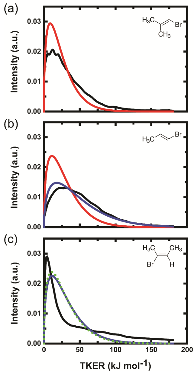
Fig. 4 Total kinetic energy release distributions corresponding to formation of HBr ( v=2, J=1 ) fragments from photolysis of (a) BMP-3, (b) EBP-34, and (c) EBB-44 at 193 nm. The black lines are experimental data after partial-slicing analysis of velocity map images. The coloured lines are statistical model predictions for the 3-C TS (solid red), 4-C TS (solid blue) and 4'-C TS (dotted green). The area under each curve is normalized to unity.
