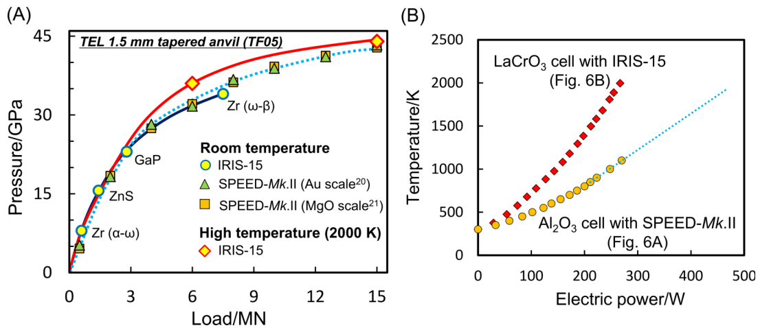
FIG. 7. (a) Pressure generation using TF05 anvils with 1.5 mm truncation and 1^\circ tapered faces at room temperature and high temperature (2000 K). Circles and diamonds are pressure generated with IRIS-15 at room temperature and 2000 K, respectively. Triangles and squares are pressure generated with SPEED-Mk.II at room temperature using equation of states of Au 20 and MgO, 21 respectively. Dotted line was drawn using triangles and squares. ZnS, GaP, and Zr were pressure calibrants at room temperature. TEL, truncated edge length. (b) Comparison of heating efficiencies of Al 2 O 3 (Fig. 6(a)) and LaCrO 3 (Fig. 6(b)) cells. Circles and diamonds are correlations between the supply power to the heater and temperature of sample part in Al 2 O 3 (Fig. 6(a)) and LaCrO 3 (Fig. 6(b)) cells, respectively. Electric powers extrapolated with those between 850 and 1100 K (dotted line) were supplied above 1100 K because thermocouple broke above 1100 K.
