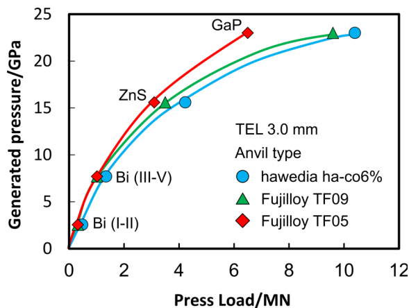
FIG. 4. Comparison of pressure generation at room temperature using carbide material hawedia ha-co6%, Fujilloj TF09, and Fujilloj TF05 with 3.0 mm truncation. Bi, ZnS, and GaP are pressure calibrants at room temperature. Solid circles, triangles, and diamonds are the results by hawedia ha-co6%, Fujilloj TF09, and Fujilloj TF05 anvils, respectively. TEL, truncated edge length.
