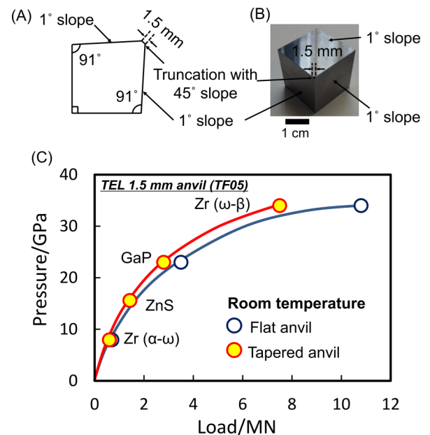
FIG. 5. Comparison of performances on pressure generation of flat and tapered anvils with 1.5 mm truncation (Fujilloj TF05) at room temperature. (a) and (b) Tapered anvils with 1.5 mm truncations as seen from [100] direction and [111] direction, respectively. (c) Pressure calibration curves at room temperature with flat and tapered anvils. ZnS, GaP, and Zr were pressure calibrants at room temperature. Solid circles and open circles are the results by flat and tapered anvils, respectively. TEL, truncated edge length.
