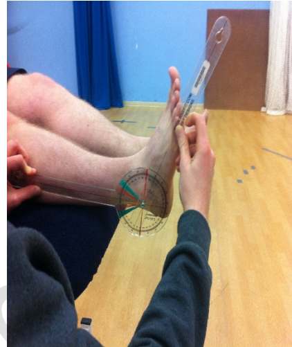
Figure 2. A-JPS DF
