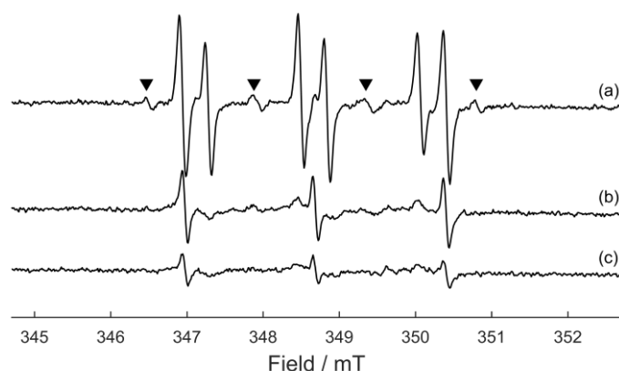
Fig. 3. X-band CW EPR spectra of L-his powder dissolved in water with a) MNP (final conc. 20 mM) added 3 minutes after dissolution and transferred using a syringe with metal needle; b) aqueous EDTA (1 mM) followed by processing as described in a); c) same as a) but transferred by using a glass Pasteur pipette. In a) the low-intensity four line EPR spectrum with a 1:2:2:1 pattern, indicated by ▼, was attributed to the spin-adduct MNP-OH (see Fig. S5 and Table S1). The EPR parameters used to record the spin-adduct spectra were as detailed in section 2.4, with number of points 1024.
