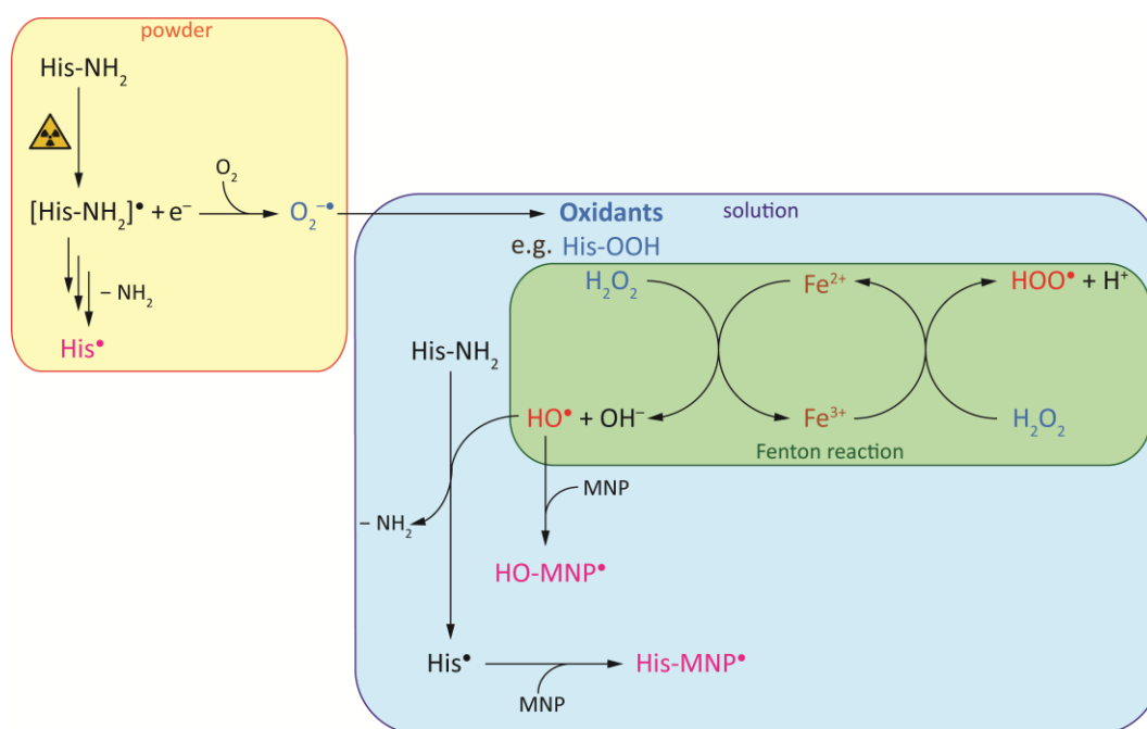
Scheme 2. Irradiation of L-his powder with formation of strong oxidants (labelled in blue) involved in the regeneration of L-his radicals in solution. The ROS produced from the Fenton reaction (in red) are scavenged by L-his, with the consequent formation of L-his radicals readily trapped by MNP to form species detected by EPR (magenta).
