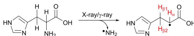
Scheme 1. Radiolytic deamination of L-his.
