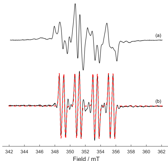
Fig. 1. a) X-band CW EPR spectrum of L-histidine (L-his) powder after \gamma -irradiation at r.t. with a total dose of 25 kGy. b) X-band CW EPR spectrum of L-his single crystal with the magnetic field aligned parallel to the c -axis after X-irradiation at r.t. (black) and EasySpin (Stoll and Schweiger, 2006) simulation (dashed red). The EPR parameters used to record the powder & single crystal spectra respectively were: a) time constant 81.92 ms; number of points 1024; number of scans 4 and b) time constant 40.96 ms; number of points 2048; number of scans 20, with other parameters as in section 2.4.
