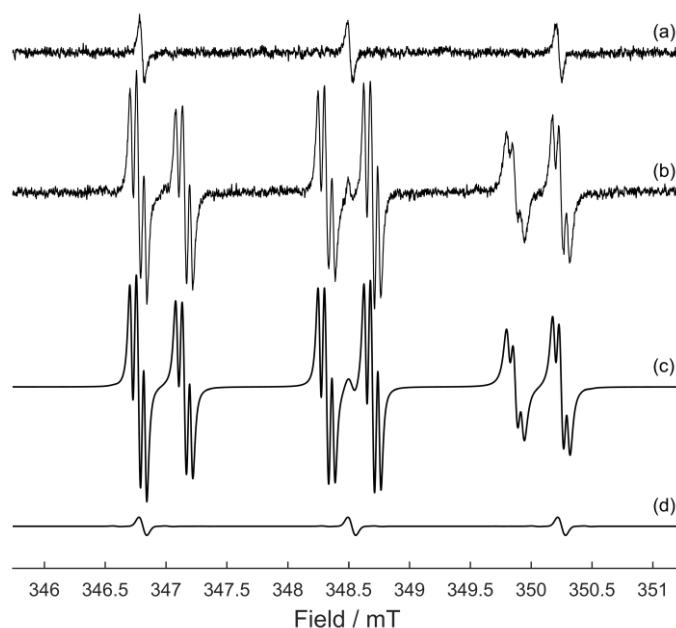
Fig. 2. X-band CW EPR spectra of a) non-irradiated L-his powder dissolved in a spin-trap solution of MNP (80 mM), b) 250 kGy \gamma -irradiated L-his powder dissolved in a spin-trap solution of MNP (80 mM), c) simulated EPR spectrum (obtained using EasySpin (Stoll and Schweiger, 2006)) for a combination of the MNP-his adduct and DTBN, and d) simulation of DTBN only. The EPR parameters used to record the spin-adduct spectra were as detailed in section 2.4 with the exception of the lower modulation amplitude of 0.01 mT; the number of points was 4096.
