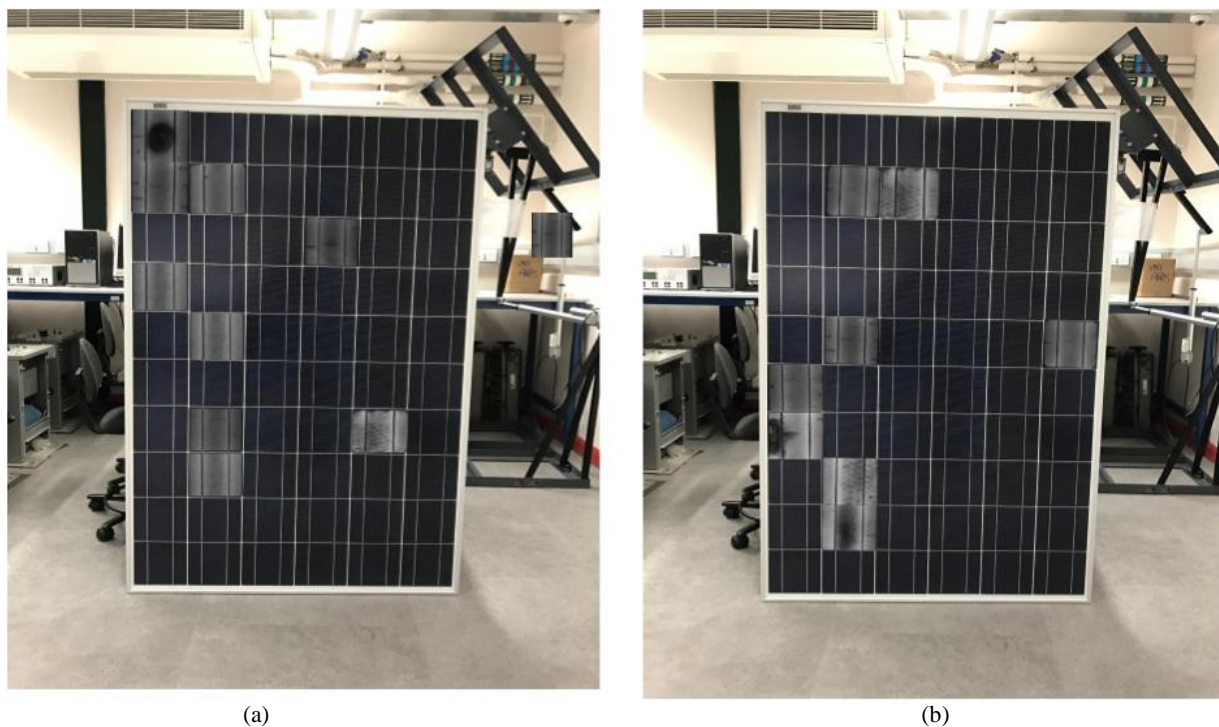
Fig. 6 EL images of cracked solar cells combined with the real images of the examined PV modules (a) PV4 - output efficiency 85.73% (b) PV7 - output efficiency 80.73%
