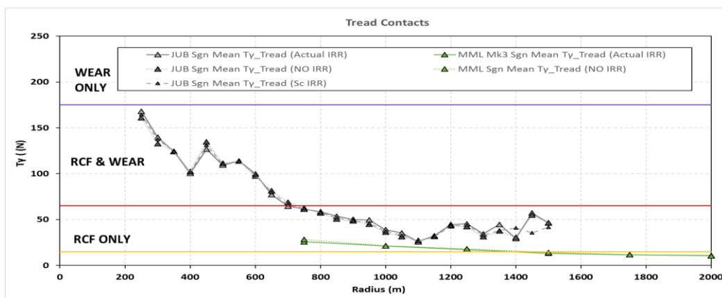
Figure 12: Effect of track irregularity on mean ‘signed T_\gamma ’ at tread contacts (Note: Actual IRR = measured TRV data, No IRR = No irregularities and Sc IRR = Scaled irregularities)
