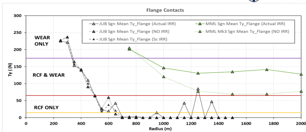
Figure 11: Effect of track irregularity on mean ‘signed T_\gamma ’ at flange contacts (Note: Actual IRR = measured TRV data, No IRR = No irregularities and Sc IRR = Scaled irregularities)
