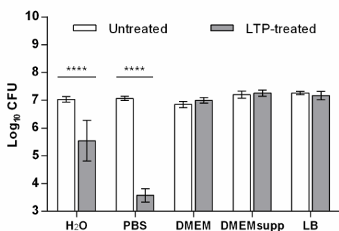
Fig. 2. Effect of external organic content on bacterial viability. CFU Log 10 reduction of S. Typhimurium in the 5 solutions exposed to plasma. Data presented as mean ± S.D. ****: P<0.0001.
