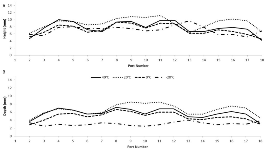
Figure 22- How temperature affects bulb size along a GDU
