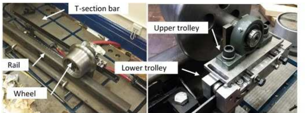
Figure 3- set up of test rig
