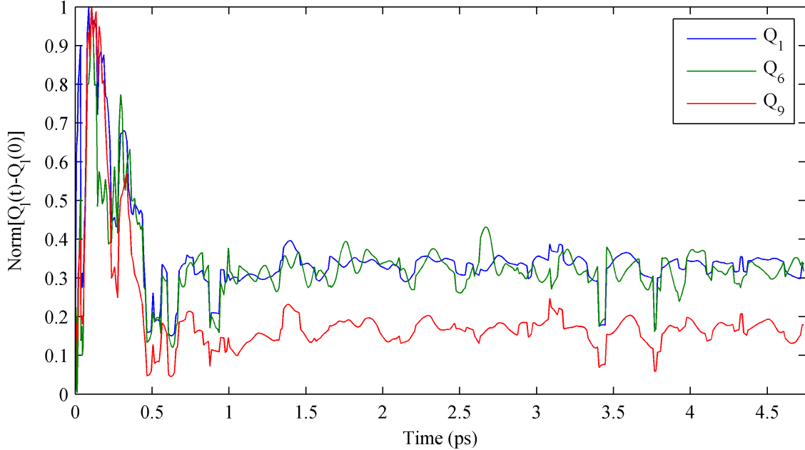
Figure 4: The time evolution of Q_1 , Q_6 and Q_9 for the zirconium species. The plot demonstrates the values of Q_l(t) - Q_l(0) normalized to give unit maxima. These three were the only SOP that presented a damaged-like behavior.
