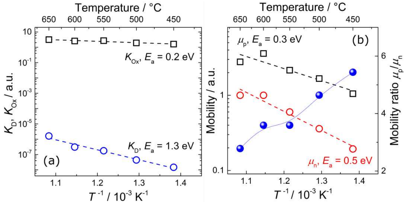
Figure 6. Optimized parameters describing the bulk properties of \text{BiFeO}_3 . (a) The equilibrium constants K_{Ox} and K_D show thermally activated behaviour. (b) Both hole and electron mobility show an activated behaviour, with \mu_p > \mu_n in the investigated temperature range. The mobility ratio \mu_p/\mu_n (blue filled circles) is around 4 and decreases with increasing temperature.
