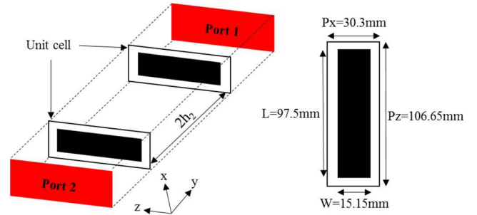
Fig. 4. Unit cell of PRS for waveguide analysis.
