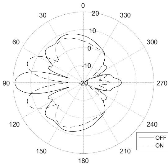
Fig. 6. Simulated farfield gain pattern (H-plane/xy-plane) at 1.842GHz, when h_2 = \lambda/2 , for the “on” and “off” PIN diode states.
