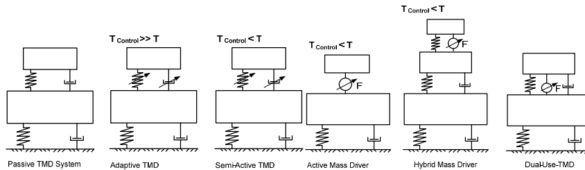
Fig. 1. Types of Control Systems – Dual Use TMD compared to passive, semi-active, active and hybrid systems
