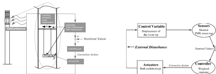
Fig.5 Feedback control loop practice.
