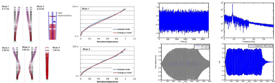
Fig. 3- Left: Relevant modes and calculated natural frequencies for model calibration – mode shape comparison – Right: Above: generated time history for the crosswind loading and resulting FFT spectrum – Below: Tower Displacement with and without optimized TMD and resulting TMD displacement
