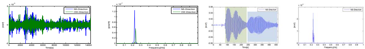
Fig. 6. Above-Left: Time History of the measured acceleration at the top of the tower in the two main directions – Above-Right: corresponding APS spectra Below-Left: Time histories of the occurring accelerations at the tower top during the artificial excitation (marked green: sinusoidal excitation / marked blue: controlled excitation mode with suppression in one of the main axis – Below-Right: FFT spectrum
