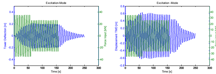
Fig.4. Numerical Time Domain Analysis – Left: Resulting tower deflections from the shown force input/Right: Resulting TMD mass displacements
