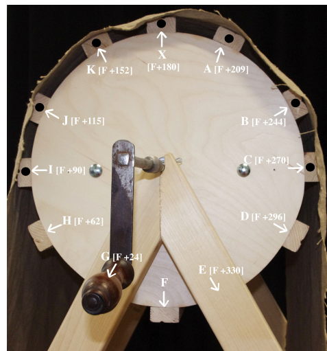
Figure 2: Placement of slats on the acoustic wind machine. A black dot marks each of the seven positions where the slats make contact with the cloth at any one time.
