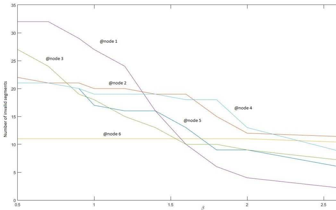
Fig. 9: Variation in number of invalid trajectory segments with respect to various nodes/regions of the RAG verses \beta value.
