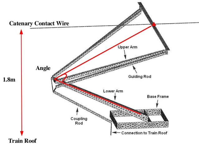
Fig. 11. The arc length changes by the varying angle of pantograph
