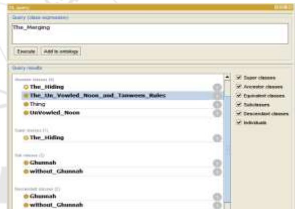
Figure13: The_Merging Query Result
