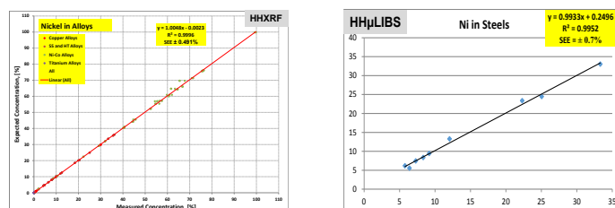
Figure 1. Example of analytical performance for nickel in alloys: HHXRF and HHuLIBS.
