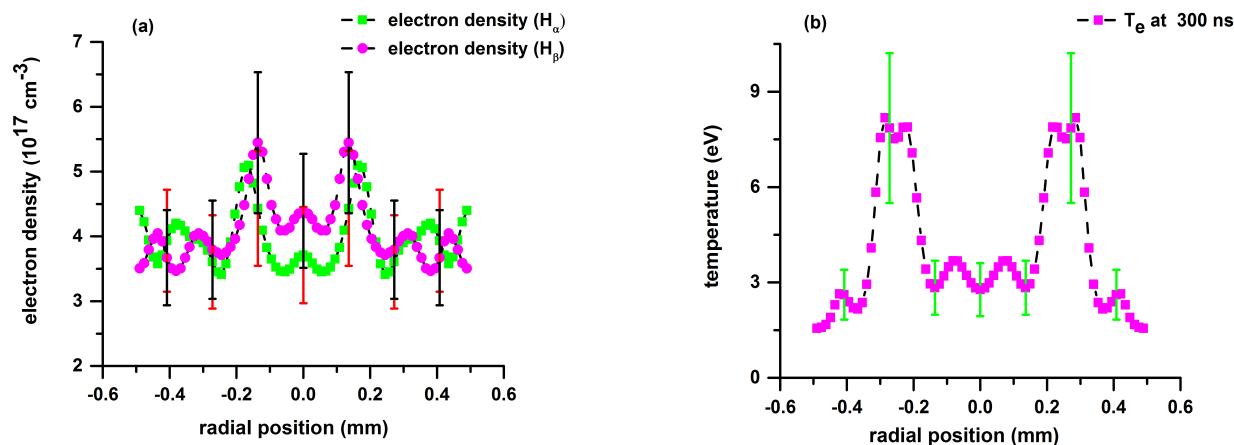
Figure 1: (a) Radial electron density and (b) temperature distribution at 300 ns time delay from optical breakdown. The measured hydrogen Balmer H \alpha and H \beta lines are used to determine [2] the spatial variation of electron density, N_e , and temperature, T_e . The radial temperature distributions are deduced from Boltzmann plots using H \alpha and H \beta lines [3-5]. The temperature in the central region of the plasma is found to be lower than found towards the outer region of the spherical ring or shell structure. The kernel expansion speed is close to the speed of sound in hydrogen gas and reveals high peak temperatures. The plasma expansion appears to be isentropic, characterized by T/N_e^{2/3} = \text{constant} , in agreement with previous hydrogen experiments [6,7].
