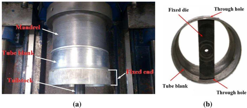
Fig. 6 Tube spinning experiments. (a) Tube blank on the mandrel. (b) The assembly of the fixed die and blank
