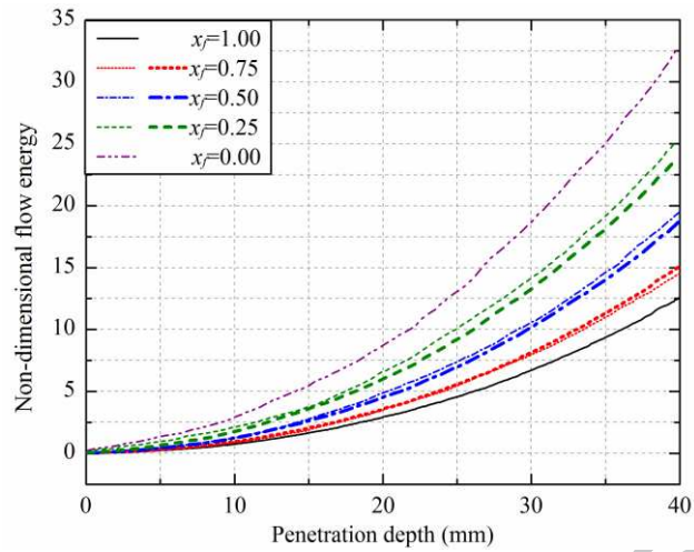
Fig. 12. The variation of the flow energy of mixtures (AR=1.5 & AR=0.0 at volume fraction, x_f , of spherical beads) with the penetration depth (thin lines: simulated results; thick lines: Eq. (6) with simulated E of the mixture).
