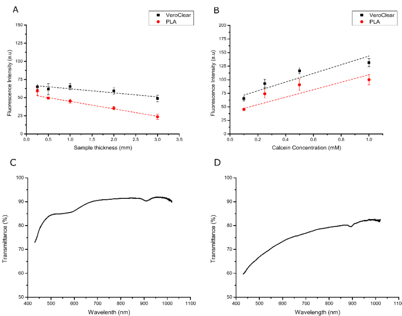
Figure 3: Transparency measurements. (A) The effect of 3D printed substrate thickness on its transparency using 1 \mu L 0.1 mM calcein droplets ( n \geq 3 ). (B) Fluorescence intensity of 1 \mu L droplets with varying calcein concentrations on different materials ( n \geq 3 ). (C)-(D) Plots of optical transmittance of VeroClear (C) and PLA (D) as a function of wavelength using 2 mm thick samples.
