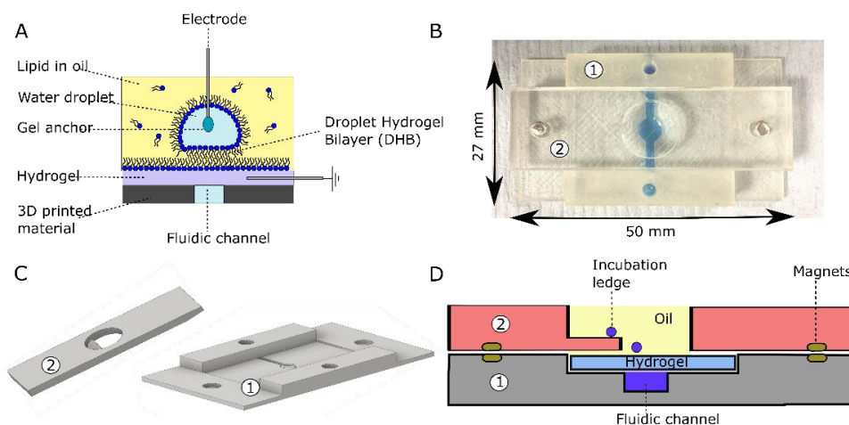
Figure 2: Transparent 3D printed device for DHB assembly. (A) Schematic of bilayer formation and current measurements via agar coated Ag/AgCl electrodes. (B) Photograph of 3D printed device with blue dye in the fluidic channel. A hydrogel sheet is sandwiched between components 1 & 2, which are held together using magnets. (C) 3D CAD image of the two 3D printed components (D) Schematic of device cross section.
