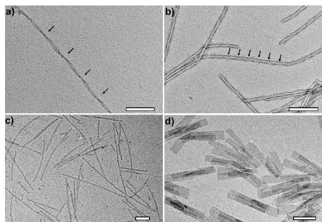
Figure 4. TEM images of nanostructures: (a) F4C11, (b) F5C11, (c) V6C11, and (d) F6C6. Scale bar: (a–c) 100 nm, (d) 500 nm. The arrows in (a) and (b) denote helical features of F4C11 and F5C11 fibrils, respectively.
