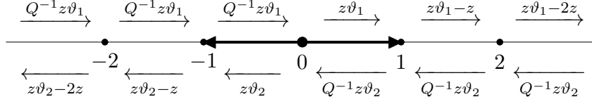
Figure 1. \mathcal{M}_{\text{red}}(\Sigma_{\mathbb{P}^1})
