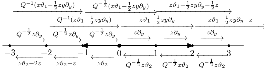
Figure 2. \mathcal{M}_{\text{red}}(\Sigma_{\mathbb{P}(1,2)}, \{1\})
