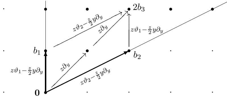
Figure 3. \mathcal{M}_{\text{red}}(\Sigma_{[\mathbb{C}^2/\mu_2]}, \{(1, 1)\})
