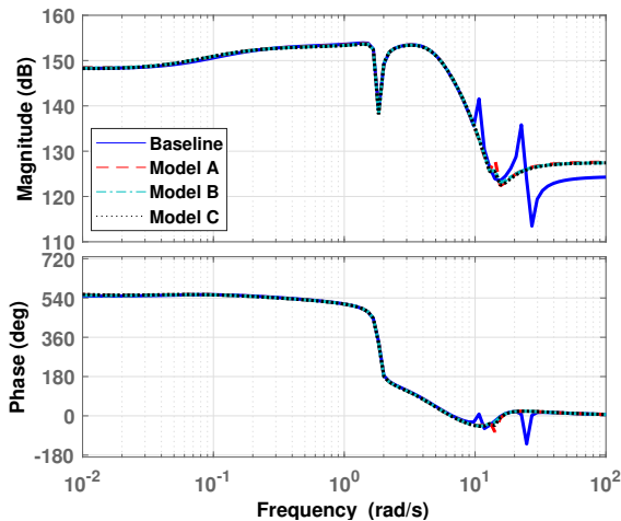
Fig. 9. From pitch angle to blade root bending moment at 15 m/s
