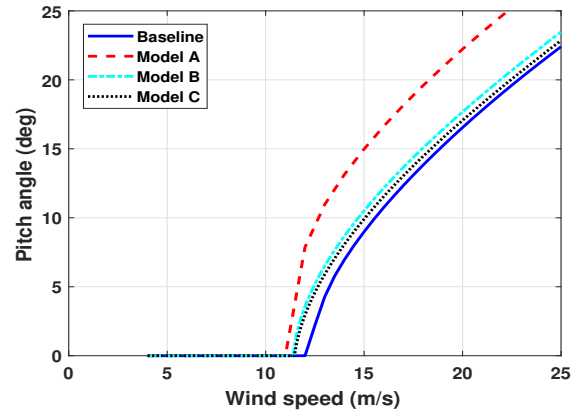
Fig. 5. Pitch angle without control
