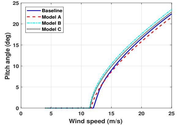
Fig. 6. Pitch angle with baseline control
