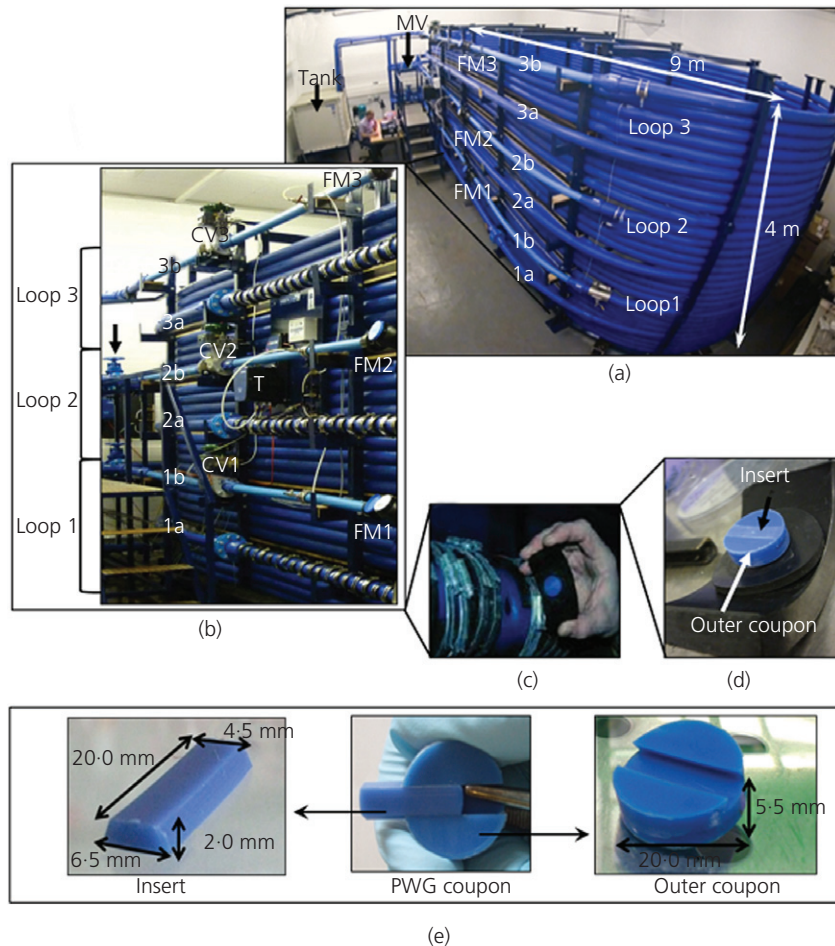
Figure 1. DWDS simulation pipe facility and Pennine Water Group (PWG) coupon. (a) Test facility: total volume (tank and loops), 4.5 m 3 ; tank volume, 1.53 m 3 ; each loop comprised nine and a half 21.4 m long coils of 79.3 mm internal diameter HDPE, with a total length of ~200 m; MV=manual valves used to separate the three loops; 1a, 2a and 3a indicate the fifth coil of each loop into which PWG coupons were inserted; 1b, 2b and 3b indicate the 50 mm internal diameter pipes containing flowmeters (FM) and control valves. (b) Detail of loop arrangement: T=turbidity meter (measured using a Chemtrac TM2200 turbidity instrument (Chemtrac Inc., USA)); CV=control valve. (c) Coupons secured in the apertures. (d) HDPE PWG coupon and rubber gasket to ensure a watertight fit. (e) PWG coupon components (insert for microscopy and outer coupon for molecular analyses) and dimensions (reproduced from Fish et al. , 2015)
