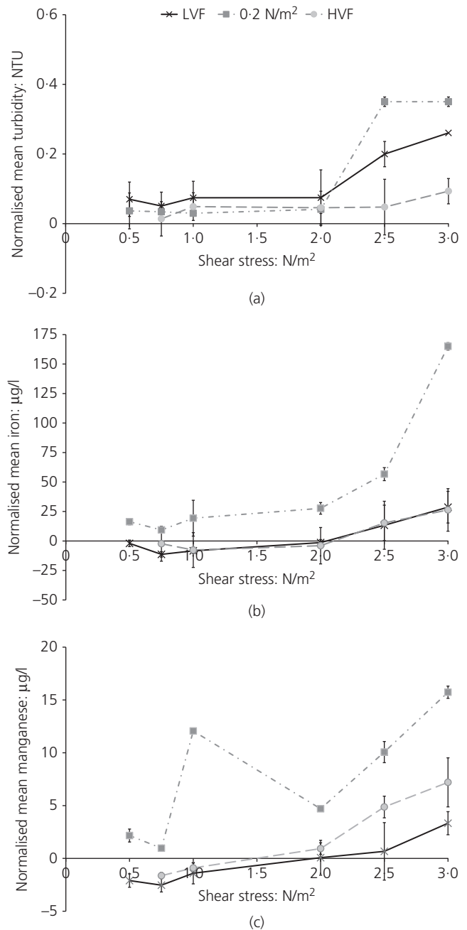
Figure 4. Comparison of normalised mean (a) turbidity, (b) iron and (c) manganese concentration during the flushing phase for loops conditioned by low varied, steady-state (0.2 N/m 2 ) and high varied hydraulic conditions
