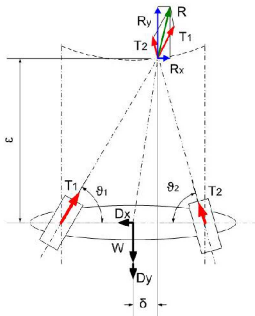
Figure 4. A preliminary model derived from Coanda patent [2]
