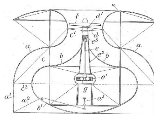
Figure 5. Aeronautical Machine by Robinson [5]
