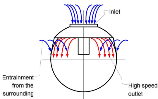
Figure 1. Preliminary concept drawing
