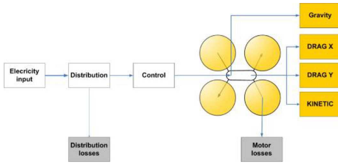
Figure 20. Energy dissipations in a multicopter
