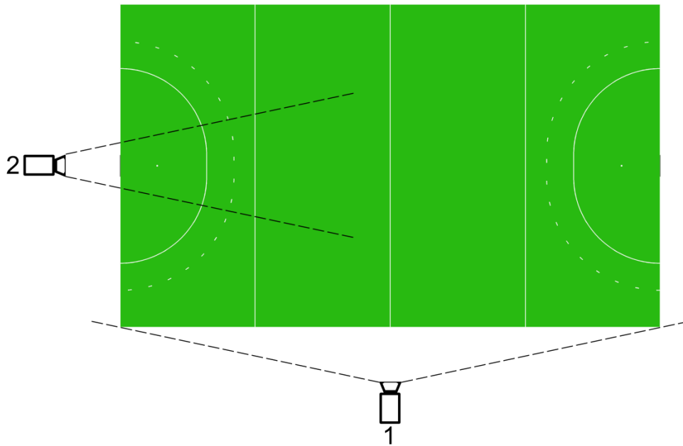
Figure 3.2 Schematic of camera locations. Camera 1 is a 4K camera with 0.3x fisheye lens. Camera 2 is a high-definition camera with a standard lens.
