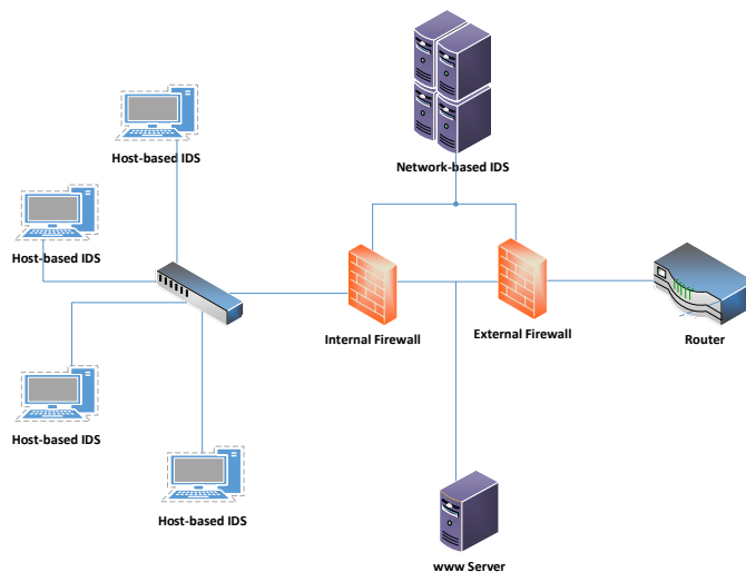
Figure 1. Signature-based IDS
