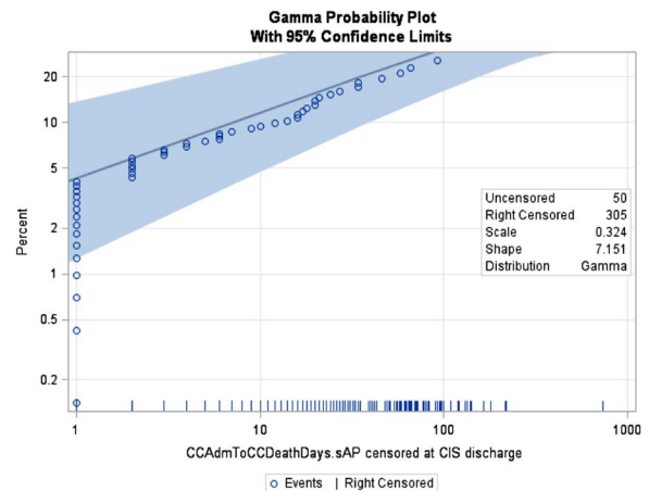
Figure 2 Probability plot (gamma model) of risk factors for death after admission to critical care. CC, critical care; sAP, severe acute pancreatitis.
