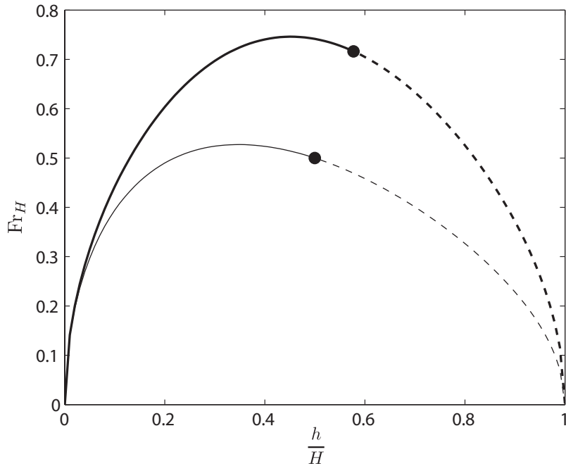
FIGURE 2. Dependence of Froude number, Fr_H \equiv U_0/\sqrt{g'H} , on the relative downstream height of the gravity current propagating horizontally in a rectangular channel (thin line) and, from (2.2), in a V-shaped valley (thick line). Solid circles indicate values for energy-conserving gravity currents and dashed lines denote unrealizable values that require external energy to maintain the flow. Note that for a current in a V-shaped valley, Fr_H is independent of the valley spread and tilt, \varphi and \phi , respectively.
