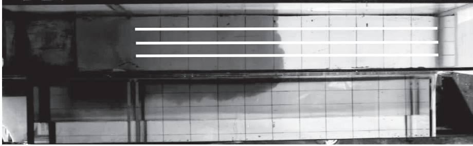
FIGURE 4. Snapshot taken from an experiment of a gravity current propagating along a horizontal rectangular channel in an ambient fluid of depth H_0 = 15.5 cm and with reduced gravity g' = 6.57 cm/s 2 . The upper part of the image shows a top-view looking through the surface of the (clear) ambient fluid to the dyed current whose front is situated approximately 50 cm to the right of the gate. The bottom part of the image shows the side view of the current visualized by a mirror tilted at 45° from the horizontal along the length of the tank. The three white lines indicate where along-tank slices were taken to construct time-series images of the rightward-advancing current front.
