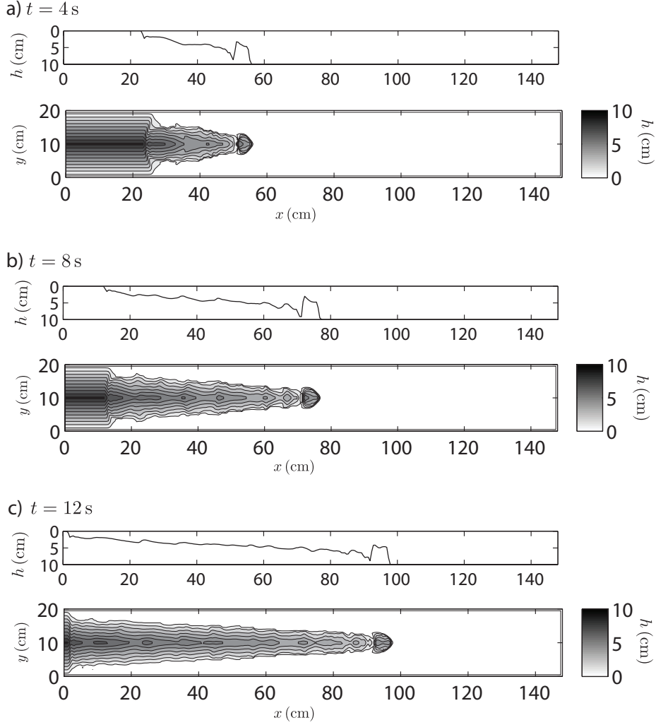
FIGURE 11. Structure of a horizontally propagating gravity current in a V-shaped valley with tilt \phi = 45^\circ as determined from simulations at times a) t = 4 s, b) t = 8 s and c) t = 12 s after release from the lock. In each case the top plot shows the current height along a vertical cross-section at y = 0 (the deepest part of the domain) and the bottom plots shows contours of current thickness as a function of along-tank ( x ) and across-tank ( y ) co-ordinates. The scale determining the depth is indicated to the right of each bottom plot.
