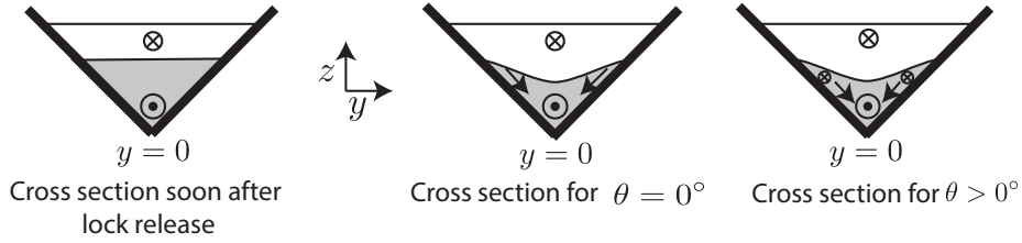
FIGURE 7. Schematic spanwise cross-section of the tilted tank showing the gravity current in gray and ambient flow in white near the gate (left) and further downstream when propagating without a slope (middle) and when flowing upslope (right).
