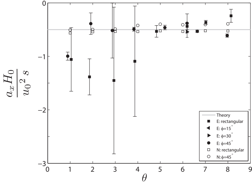
FIGURE 9. As in figure 8, but plotting the (negative) acceleration of the current normalized by u_0^2 s/H_0 , in which u_0 is the horizontal component of the front speed measured shortly after the current was released from the lock, as shown in figure 6.
