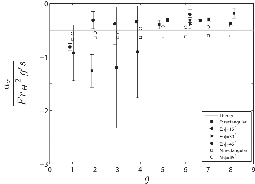
FIGURE 8. Horizontal component of the (negative) relative acceleration, a_x / (Fr_H^2 g' s) , versus the rise-angle, \theta . Here Fr_H is the Froude number predicted for energy-conserving currents. Values are plotted for (solid symbols) laboratory experiments and (open symbols) numerical simulations with currents in a rectangular channel indicated by squares and currents in a V-shaped valley with tilt, \phi , as indicated in the legend. The horizontal gray line is the (negative) relative acceleration predicted by theory. Errors in the measurements taken from laboratory experiments are indicated by vertical error bars.
