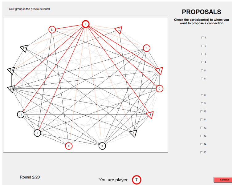
Figure 4: Linking proposals: reciprocated and unreciprocated
