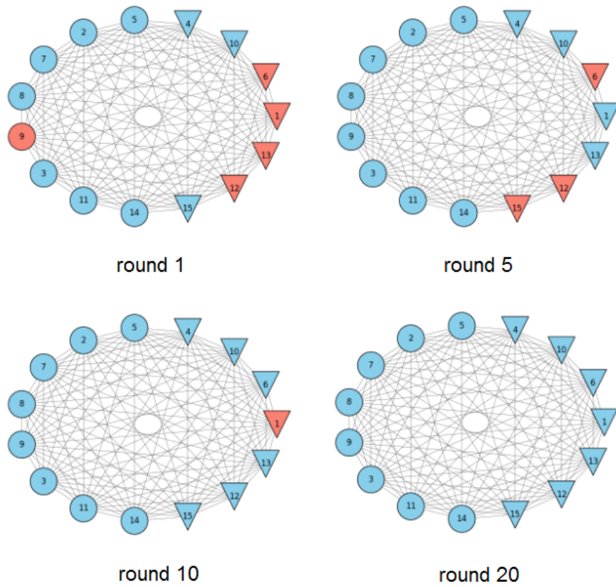
Figure 7: Illustration of dynamic behavior in EXO
