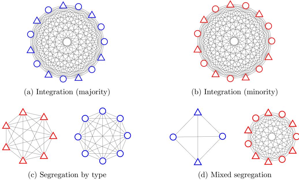
Figure 2: Pairwise stable outcomes
