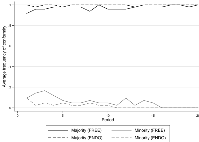
Figure 16: Action Choice in FREE vs. ENDO .
