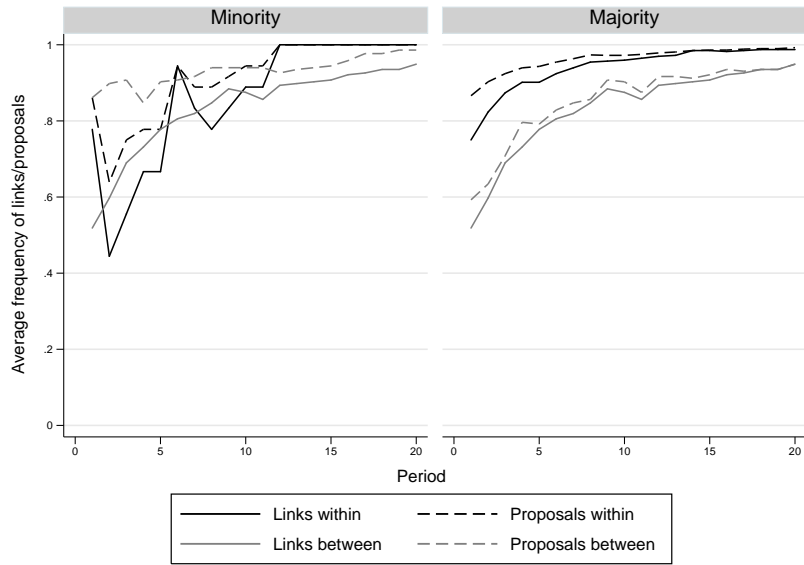
Figure 18: Link Choices under LOWCONFLICT
