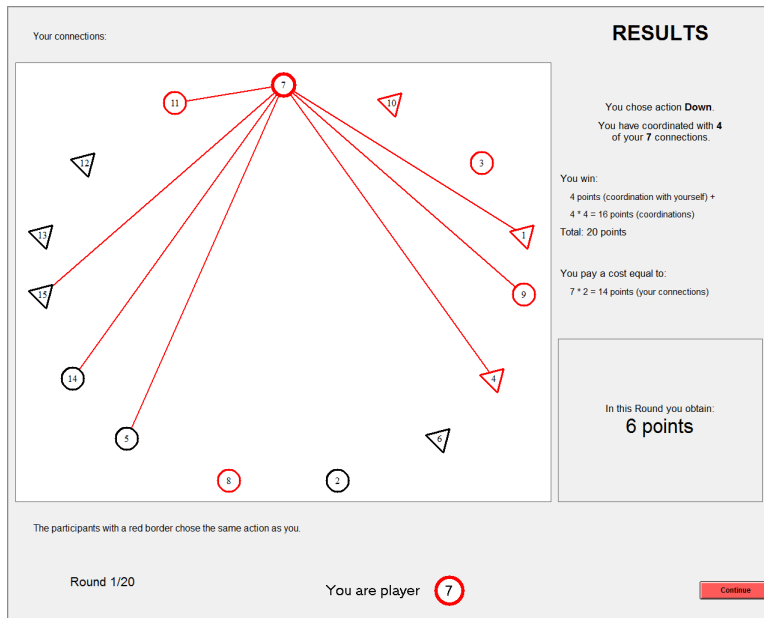
Figure 5: Neighborhood, Actions and Payoffs
