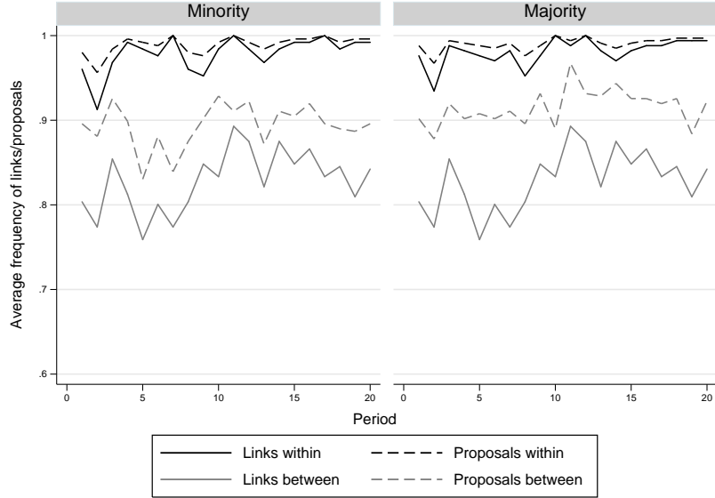
Figure 15: Link Choices in FREE .
