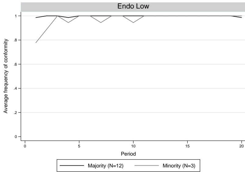
Figure 19: Action Choice under LOWCONFLICT
