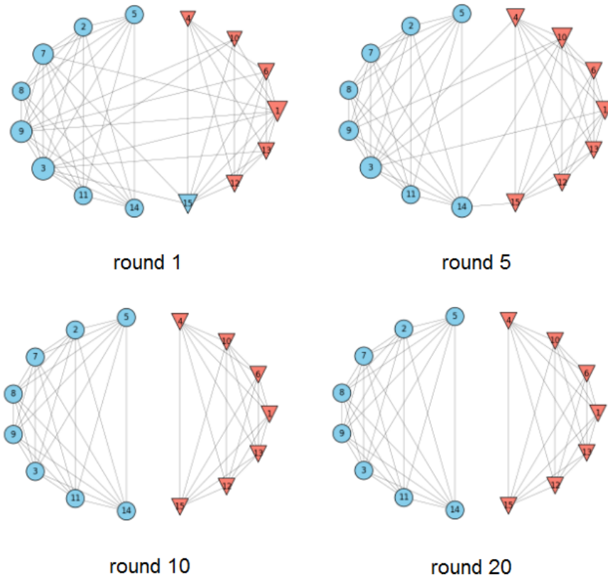
Figure 8: Illustration of dynamic behavior in ENDO
