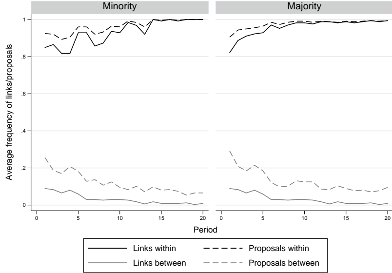
Figure 10: Link Choices in ENDO .
