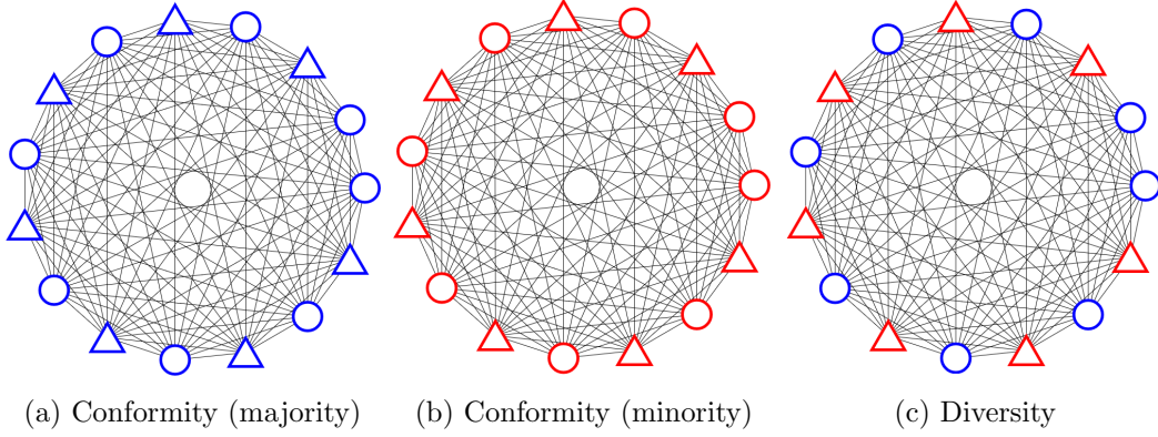
Figure 1: Nash equilibria in complete network
