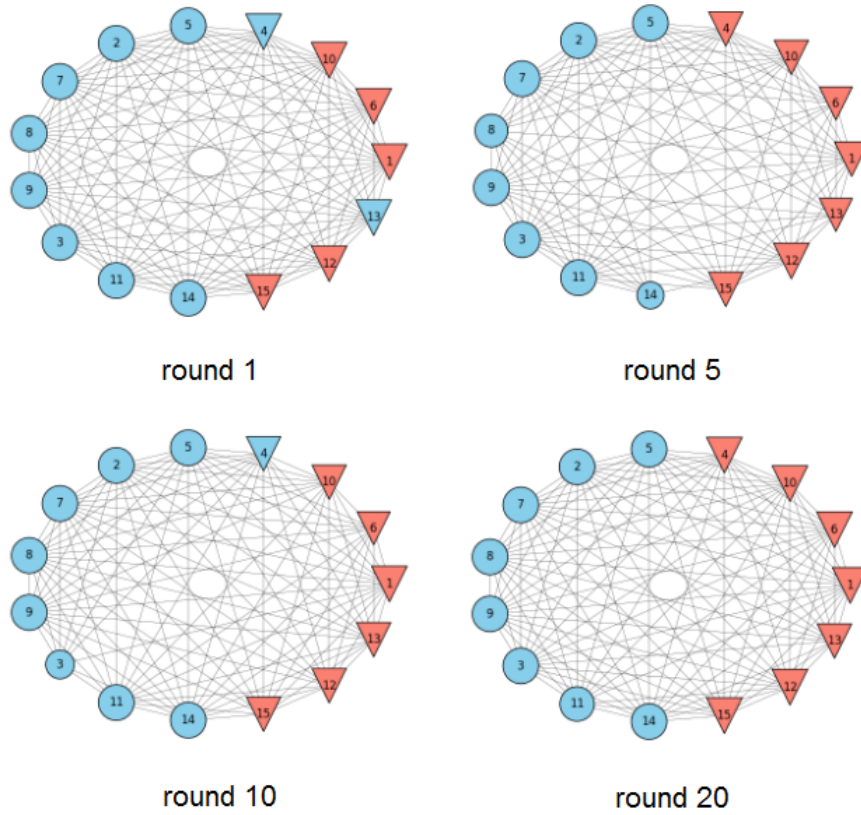
Figure 14: Illustration of dynamic behavior in FREE
