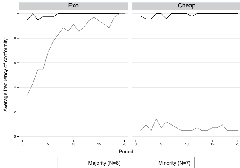
Figure 13: Action Choice in CHEAP .
