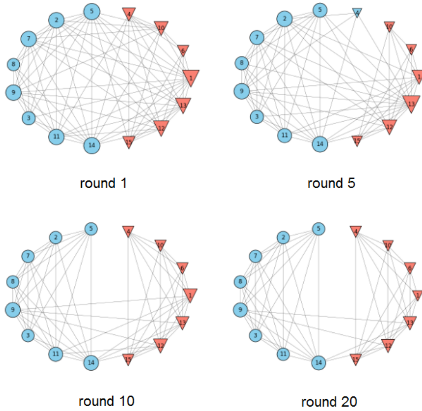
Figure 11: Illustration of dynamic behavior in CHEAP
