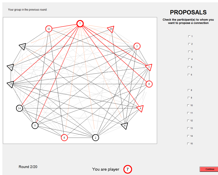
Figure 6: Feedback from previous round
