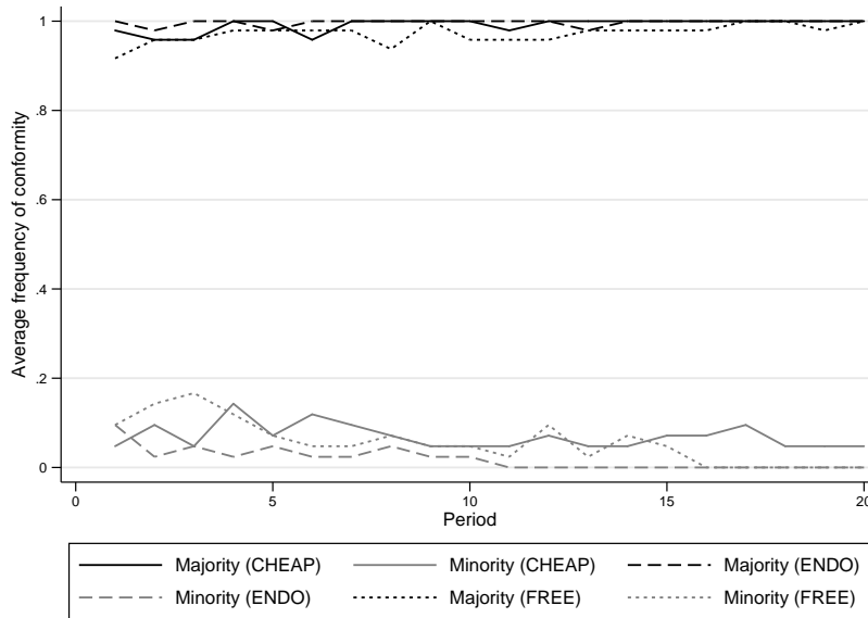
Figure 17: Action Choice in the endogenous linking treatments
