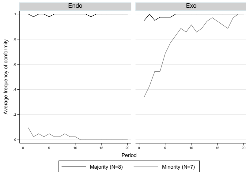
Figure 9: Action choice in ENDO and EXO .
