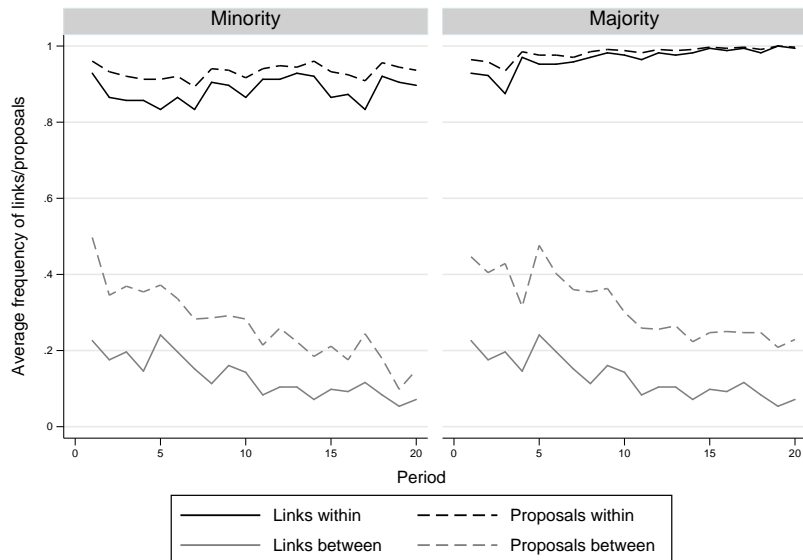
Figure 12: Link choices in CHEAP .
