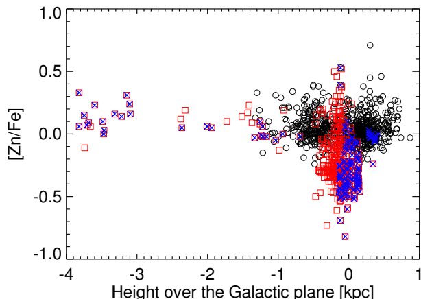
Fig. 14. [Zn/Fe] as a function of the height above (or below) the Galactic plane. Symbols as in Fig. 11.
