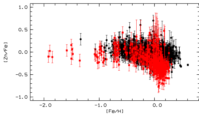
Fig. 12. [Zn/Fe] vs. [Fe/H] for the complete GES sample stars with detection of zinc. Black filled circles represent dwarf stars, red filled squares represent giant stars.
