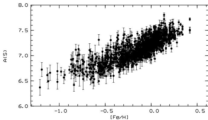
Fig. 4. A(S) vs. [Fe/H] . Error bars take into account 3\sigma uncertainty due to spectral S/N and derived by using Cayrel’s formula.
