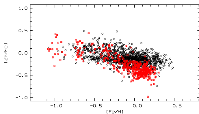
Fig. 13. [Zn/Fe] vs. [Fe/H] in the case of zinc derived with MyGIsFOS only for the 481.0 nm line. Symbols are as in Fig. 11.
