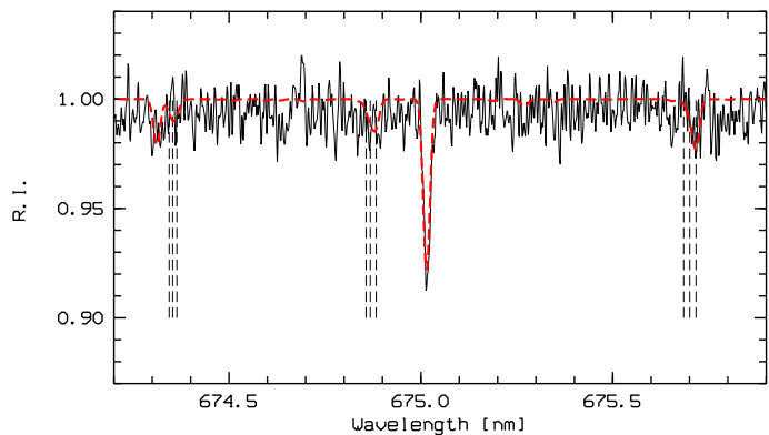
Fig. 3. The observed spectrum (solid black) of the star 21300738+1210330 in the range of the Mult. 8 of sulphur. A synthetic (dashed red) spectrum with the sulphur abundance derived of A(\text{S}) = 6.26 by the analysis is also included. Vertical dashed black lines highlight the positions of the S I lines of the Mult. 8.
