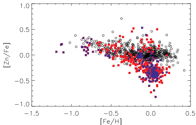
Fig. 11. [Zn/Fe] vs. [Fe/H] for the sample stars analysed for sulphur. Dwarf stars are represented as black open circles, giant stars as red squares, and stars in clusters as blue crosses.
