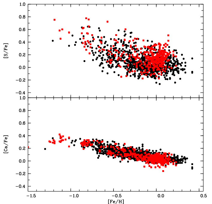
Fig. 5. [S/Fe] vs. [Fe/H] (upper panel) compared to [Ca/Fe] vs. [Fe/H] (lower panel). Black filled circles refer to dwarfs while red filled squares to giant stars. Error bars are not included for clarity, but they are presented in Fig. 6.
