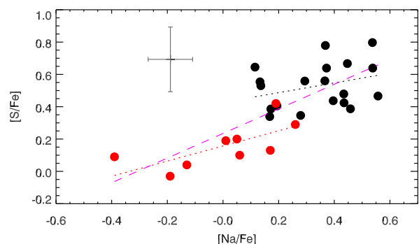
Fig. 10. [S/Fe] vs. [Na/Fe] for stars in NGC 104. Black points are GES measurements in giants, red points are Sbordone et al. (2009) TO and SGB stars, shifted to our adopted solar abundance scale. Linear fits are included, the magenta line indicating the fit to the whole sample. A conservative error estimate is also shown.
