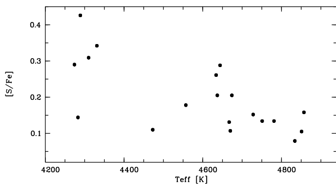
Fig. 8. [S/Fe] versus effective temperature for the 19 stars in NGC 6705.
