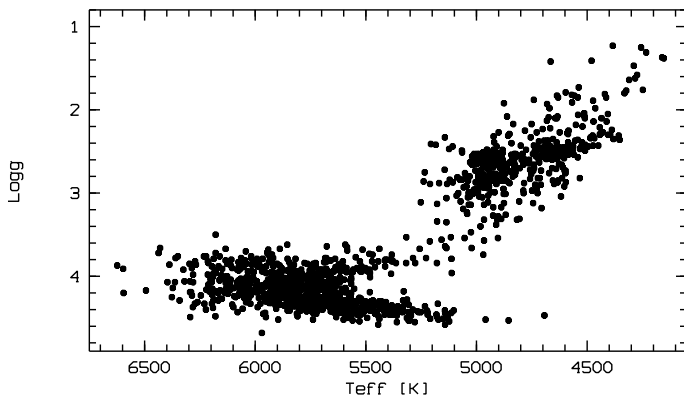
Fig. 2. The stars analysed in this work are shown in the T_{\text{eff}} vs. \log g plane.
