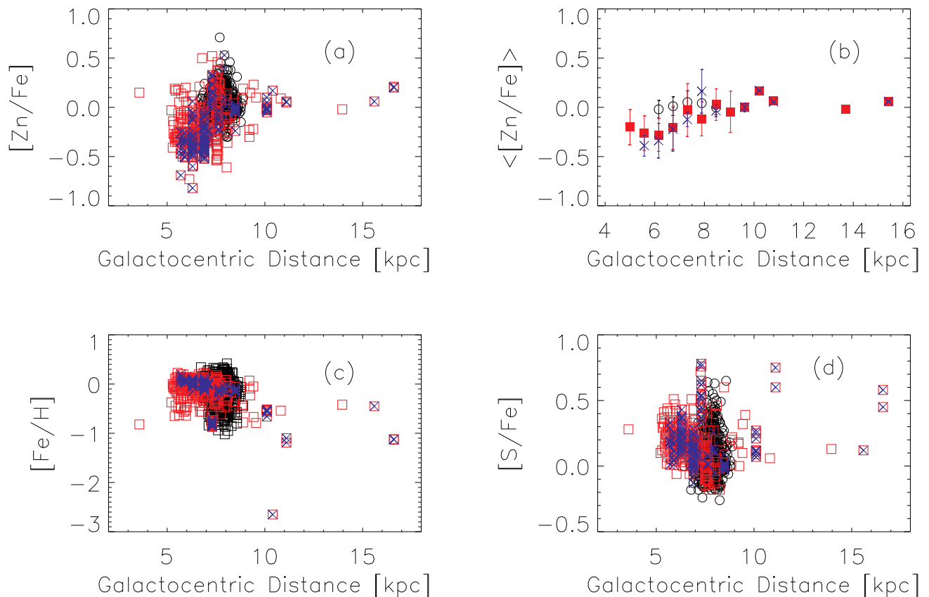
Fig. 15. Panels a, c, d : The [Zn/Fe] ( a ), the [Fe/H] ( c ), and the [S/Fe] abundances ( d ) for the sample of stars analysed for sulphur as a function of their Galactocentric distance. Symbols are the same of Fig. 11. Panel b : The average \langle [Zn/Fe] \rangle in different distance bins for dwarfs (black circles), giants (red squares) and for stars in clusters (blue crosses).
