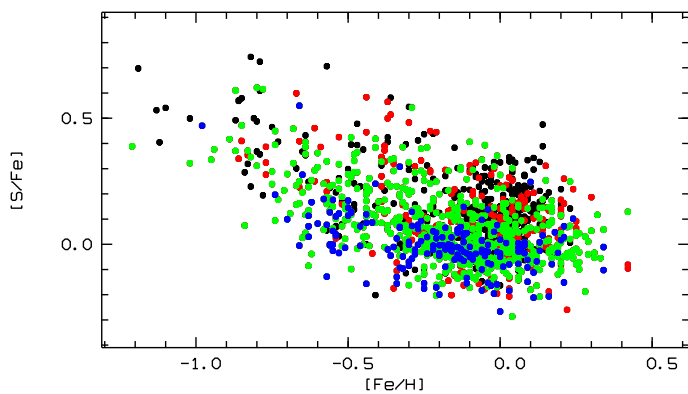
Fig. 7. [S/Fe] vs. [Fe/H] for the complete sample of stars: black, stars cooler than 5000 K; red 5000 \leq T_{\text{eff}} < 5500 K; green 5500 \leq T_{\text{eff}} < 6000 K; blue hotter than 6000 K.
