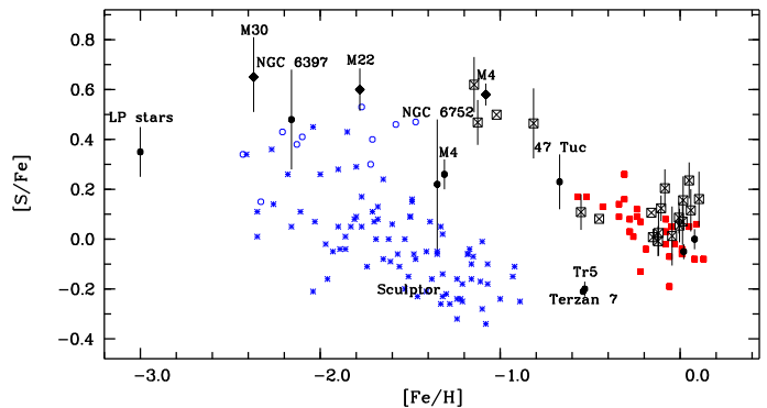
Fig. 9. [S/Fe] vs. [Fe/H] for the stars members of open and globular clusters, compared to analysis of clusters and field stars available in the literature. This is an update of figure 4 of Caffau et al. (2014), see references therein. For added samples: crossed black squares are from this work, blue stars are stars belonging to Sculptor dSph from Skúladóttir et al. (2015), open blue circles are field stars from Jönsson et al. (2011), and red filled squares are field stars from Ecuivillon et al. (2004).
