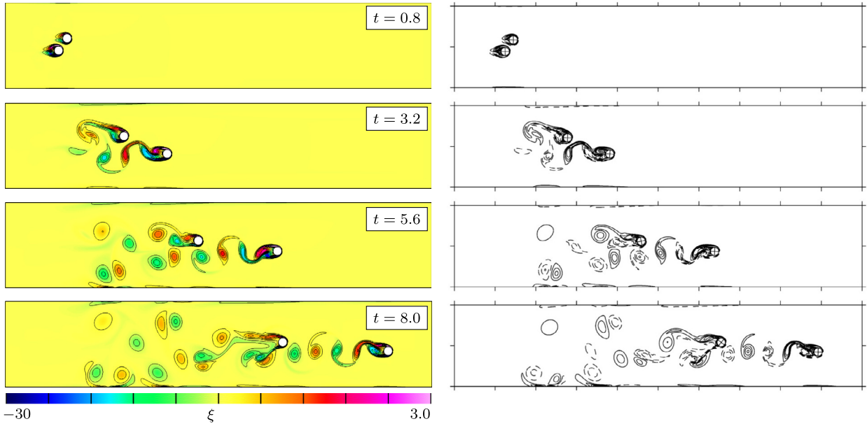
Fig. 12. Contours of vorticity at times t = 0.8, t = 3.2, t = 5.6, t = 8.0 for the pure wake interaction test case compared to plots from Uhlmann [16] taken at the same times and with the same vorticity extrema. Left: present study using a quasi-uniform grid with DLS = D/40 and SLS = D/40 . Right: results from [16] computed on a uniform grid of resolution D/40 .
