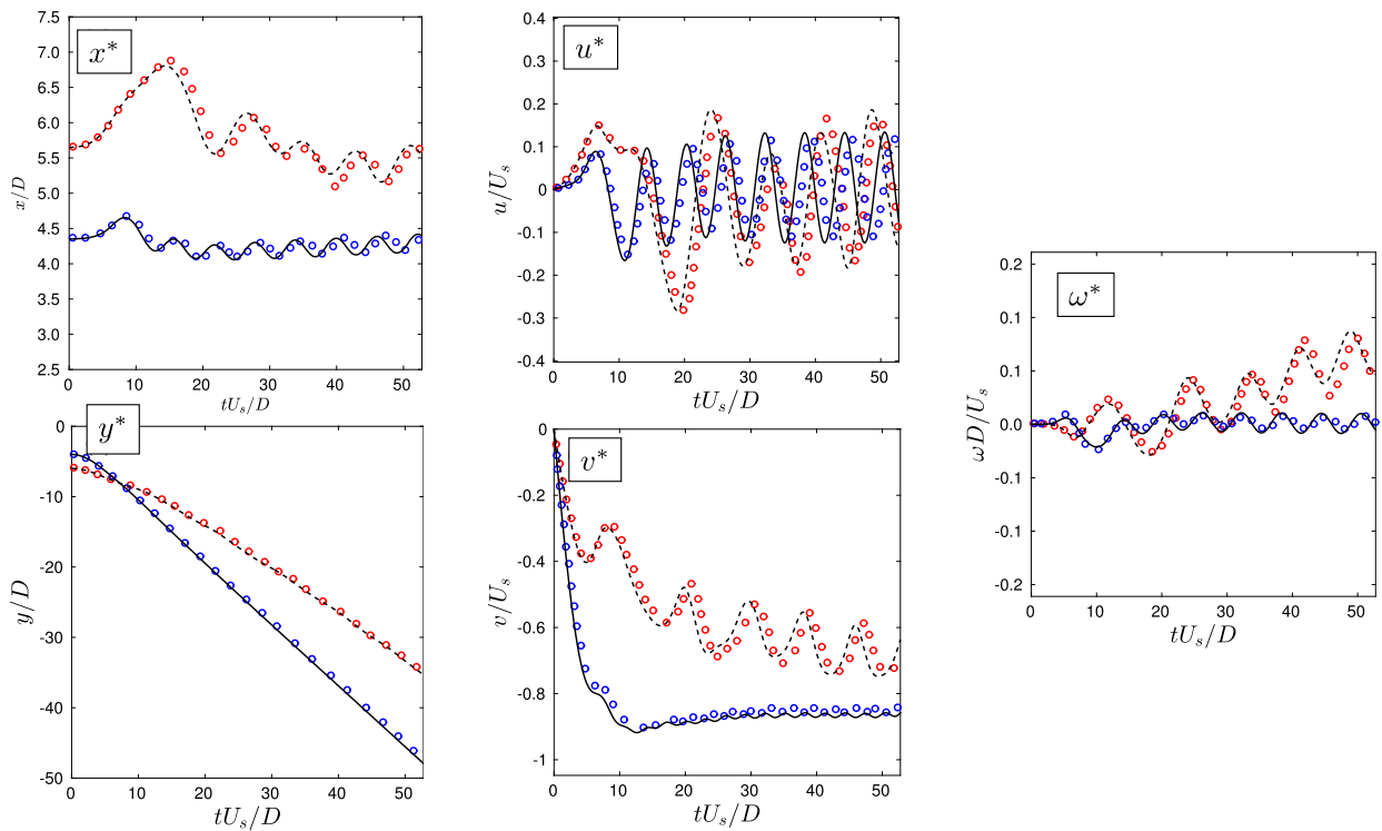
Fig. 13. Time histories of x^*, y^*, v^*, u^* and \omega^* for the pure wake interaction test case with \rho_{r,1} = 1.5, \rho_{r,2} = 1.25, \nu = 0.0008 \text{ m}^2/\text{s} and data from Uhlman [16] overlaid.
