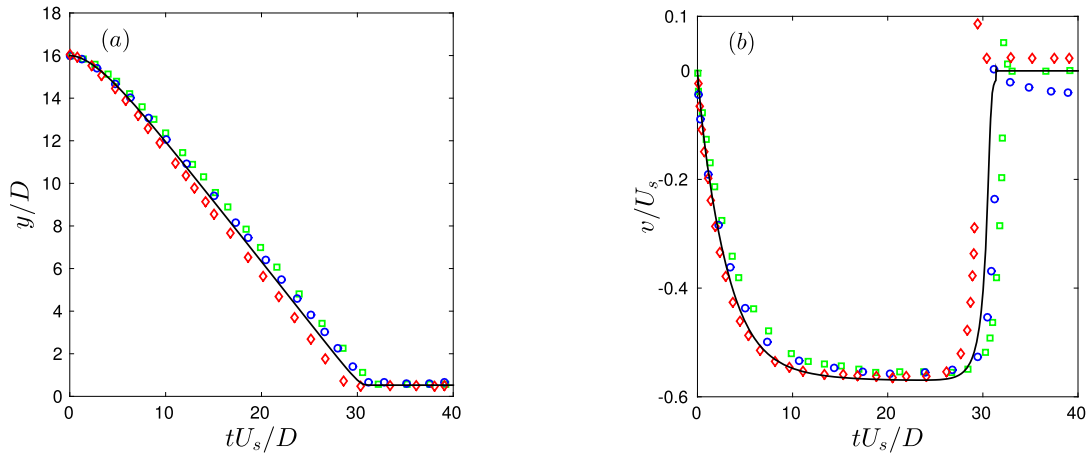
Fig. 6. Histories of the y^* -coordinate and v^* component of the centre of the disk for a low Reynolds number sedimentation of a symmetrically placed disk test case with data from Hu et al. [64] ( \square ), Wang et al. [63] ( \circ ), Glowinski et al. [13] ( \diamond ) and the present study (—).
