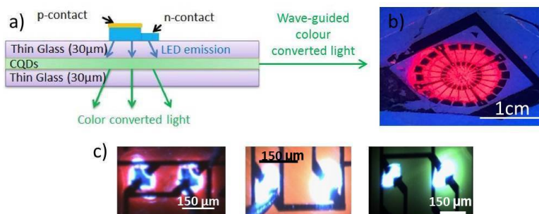
Fig. 2: a) Side view schematic of the integrated LED-color-converter device, b) oblique view of the red sample under UV illumination and c) images of the transfer printed LEDs lighting up on each of the three samples
