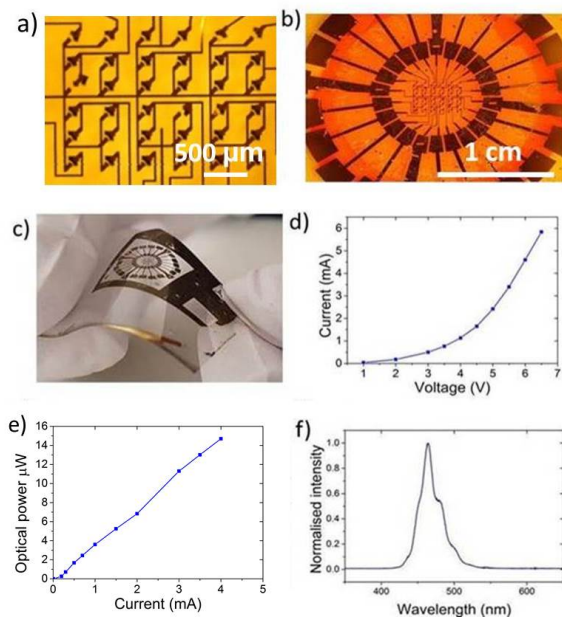
Fig. 1: a), b), c) Plan view photographs of a 6 x 6 array of \mu LEDs printed on thin glass with decreasing magnification. The \mu LEDs pictured here are 100 x 100 \mu m 2 . A typical d) IV curve, e) LI curve and f) spectrum for these \mu LEDs at a drive current of 5 mA.
