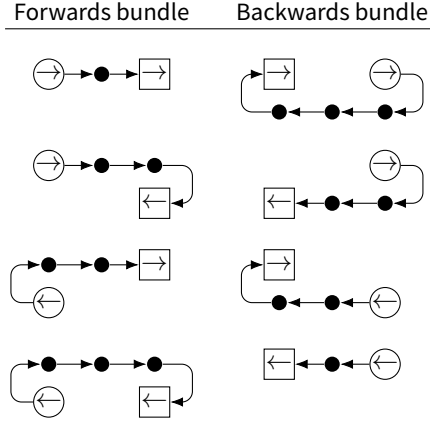
Figure 9: Dummy nodes (black dots) are needed to connect the source (circle) and target (square) of a bundle, if they are not in adjacent layers. There are eight possible combinations depending on the direction and relative placement of the source and target: for the situation drawn here, where the source and target are two layers apart, between one and three dummy nodes may be needed. This contrasts with a non-Sankey graph, where the nodes do not have a direction and only one dummy node would be needed in each case.
