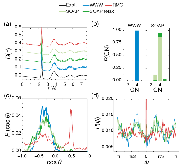
FIG. 3. Key geometric correlation functions for the different models of a -Si: WWW, the refined SOAP configuration, SOAP after relaxation, and an RMC refined configuration with no other restraints. (a) Pair distribution functions ( D(r) normalisation) including comparison to the referenced WWW-derived model, (b) the coordination number distribution P(\text{CN}) , (c) the bond angle distribution P(\cos \theta) and (d) the dihedral angle distribution P(\psi) . The dihedral angle distribution for the RMC model has been truncated as it reaches a peak of 0.077 at \psi = 0^\circ .
