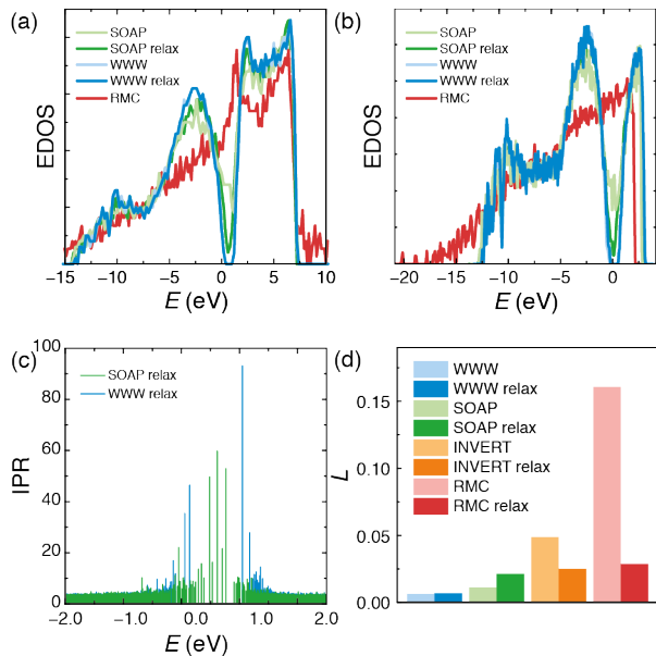
FIG. 4. (a) The calculated tight-binding (TB) electronic density of states (EDOS) for the SOAP and WWW models before and after ab initio optimisation. The density of states for the unrestrained RMC refined configuration is shown for comparison. (b) The EDOS calculated using the MBJ functional, which reproduces the same form as the TB model ( E_F = 0 for the WWW optimised model). (c) The inverse participation ratio calculated from the TB structure for the optimised SOAP and WWW configurations showing the localisation of near- and in-gap states. (d) Calculated SOAP measure L for configurations before and after optimisation show that an increase in structural quality tends to also increase the structural similarity.
