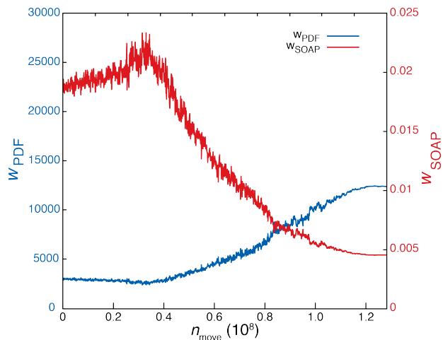
FIG. 2. Evolution of the weighting scheme for the SOAP+PDF refinement using the dynamic weighting scheme throughout the refinement as a function of proposed moves.
