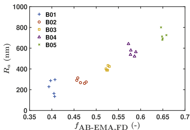
Figure 10. Roughness analysis of 5 tablets per batch as a function of the porosity. The porosity was predicted by the AB-EMA using n_{\text{eff}}(1 \text{ Thz}) from the FD analysis.
