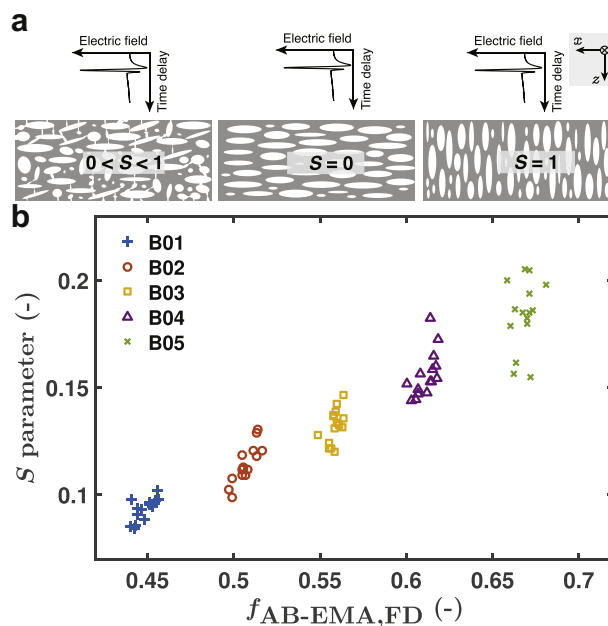
Figure 5. (a) Schematic for the interpretation of the S parameter. (b) S parameter as a function of porosity. The porosity was predicted from the AB-EMA using n_{eff} from the FD analysis. n_{FCC} (required for the calculation of the Wiener bounds in Eqs. 5 and 6) was calculated using AB-EMA and is given in Table 2.
