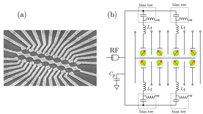
FIG. 9: (Color online) A realistic quantum dot array with triplet profile measurement: (a) SEM image of an example quantum dot array, as realised in [10]. (b) Circuit schematic of an eight dot device with dispersive gate sensors which forms a N = 8 open spin chain. The gate sensors are formed by coupling an RF-signal to gate electrodes via bias tees. L_t are chosen so that a resonant tank circuit is formed in combination with the dot system and the parasitic capacitance, C_p . The reflected RF-signal is used to read out the total capacitance of all double dots in parallel and hence m_t . The dashed blue lines denote pairings of the quantum dots for this ST-measurement.
