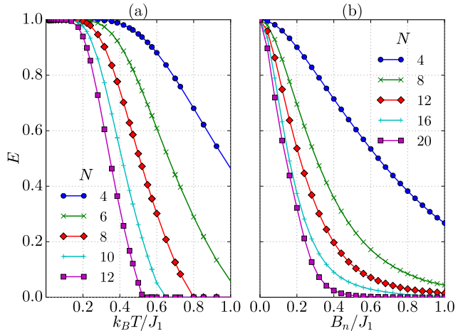
FIG. 7: (Color online) Entanglement localization to the ends of an open chain under the influence of temperature and hyperfine interactions: (a) Entanglement (as measured by concurrence) between the two furthest spins after an all-singlet measurement result on the remaining middle section of the chain, varying with temperature 1/\beta and length N . (b) The same, but now varying with the strength of the random nuclear field B_n . It is worth mentioning that a realistic (but pessimistic) estimation of the hyperfine interaction is B_n/J_1 \sim 0.1 [13]. For all considered lengths, this yields high entanglement.
