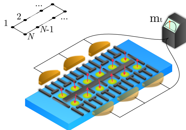
FIG. 1: (Color online) Quantum dot array spin model simulator and triplet profile readout: A simplified schematic of a quantum dot array simulating a Heisenberg N = 12 closed chain with Singlet-Triplet measurements. Here, grey bars represent voltage gates, each arrow a single confined electron, and the gold detectors Singlet Triplet measurements. These are simultaneously performed such that the total number of triplets present, m_t is recorded.
