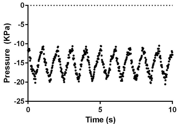
Fig 3. Representative pressure profile in the breastfeeding simulation apparatus. Values are representative of that of a suckling infant, and were measured from the breastfeeding simulation apparatus over 10 seconds occurring several minutes into a trial run testing tablet T2.
