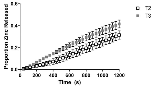
Fig 5. Release of zinc from the NSDS for Tablet Composition 2. Values are based on a weight fraction proportion; n = 3; error bars represent standard error.
