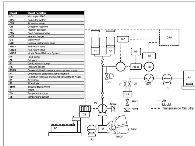
Fig 2. Breastfeeding Simulation Apparatus. (adapted from Gerrard et al., [9]).
