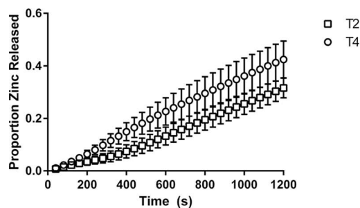
Fig 6. Release of zinc from the NSDS for Tablets of Similar Hardness. Values are based on a weight fraction proportion; n = 3; error bars represent standard error.
