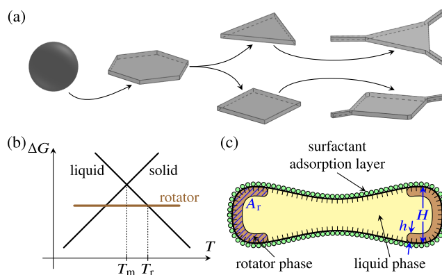
FIG. 1. Shape-shifting droplets. (a) Main stages of droplet shape evolution, following Ref. [3]. Initially spherical droplets flatten, first into hexagons, then into quadrilaterals or triangles, before growing thin protrusions. (b) Energy diagram, showing a range of temperatures close to the melting temperature where the formation of a rotator phase is energetically favored. (c) Cross section of flattened droplet. A layer of plastic rotator phase has formed at the edges of the droplet.
