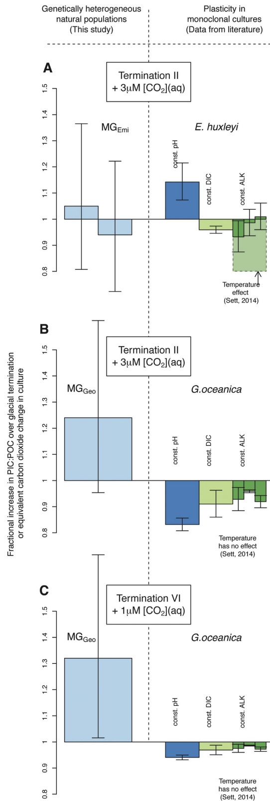
Figure 3. Fractional change in PIC:POC of natural heterogeneous populations over glacial terminations (left), compared with that of monoclonal strains subject to an equivalent CO_2 change in culture (right). (A) The response of MG_{E_{mi}} in nature is within the range of uncertainty and of plasticity of E. huxleyi observed in the laboratory. (B,C) The PIC:POC of MG_{Geo} in nature increases across both terminations, which is opposite to the equivalent plastic response as inferred from culture manipulations in G. oceanica . Error bars represent the 1\sigma uncertainty, which for the down-core response, is calculated using the prediction interval of Eq. 3. For culture results, details of the regressions are given in the Supplementary material.
