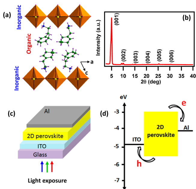
Figure 1. (a) Schematic crystal structure of 2D perovskite ( C_6H_9C_2H_4NH_3)_2PbI_4 . 14 (b) X-ray diffraction pattern of a CHPI thin film revealing a 2D-layered arrangement. (c) Schematic and (d) corresponding band diagram of the photodetector configuration 1 [Al/CHPI/ITO].
