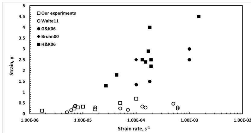
Fig. 2. Conditions used in this and previous studies of the effect of deformation on textural development in silicate-metallic melt experiments. Walte11: Walte et al. (2011), G&K06: Groebner and Kohstedt (2006), Bruhn00: Bruhn et al. (2000), H&K06: Hustoft and Kohlstedt (2006). Note that Walte et al. (2011) compressed samples axially, compared to simple shear geometry used in other studies, so determined finite shear is not strictly comparable.
