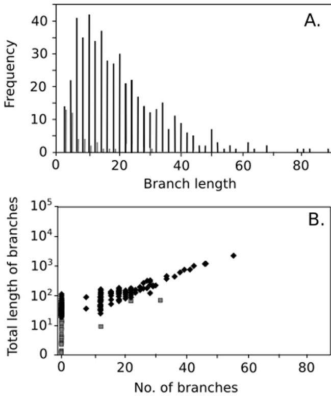
Fig. 13. Branch length analysis from skeletons of deformed and undeformed samples. A. Comparison of the distribution of branch lengths in the largest connected network of Cam3-FeO11 (black lines), and the full FeOIPC8 segmentation (grey lines). Only the largest connected network was examined in FeO11 because of the difficulty of processing all 1000 individual graphs to analyse mean length distribution. Branch length overall is much greater in the deformed sample, and the number of branches within the single deformed network is orders of magnitude greater than in the undeformed sample (made up of 18 individual isolated skeletons). This reveals the complexity of the deformed melt network, being made up of numerous larger melt pockets connected by wetted grain boundaries between numerous small olivine grains. B. Total number of branches in vs. total length of branches summed FeO11 (black diamonds) and FeOIPC8 (grey squares). Total length of branches in the deformed networks is almost 2 orders of magnitude greater than the largest skeleton observed in the undeformed sample. Lengths are in voxels, each voxel representing a length of 0.13 \mu\text{m} .
